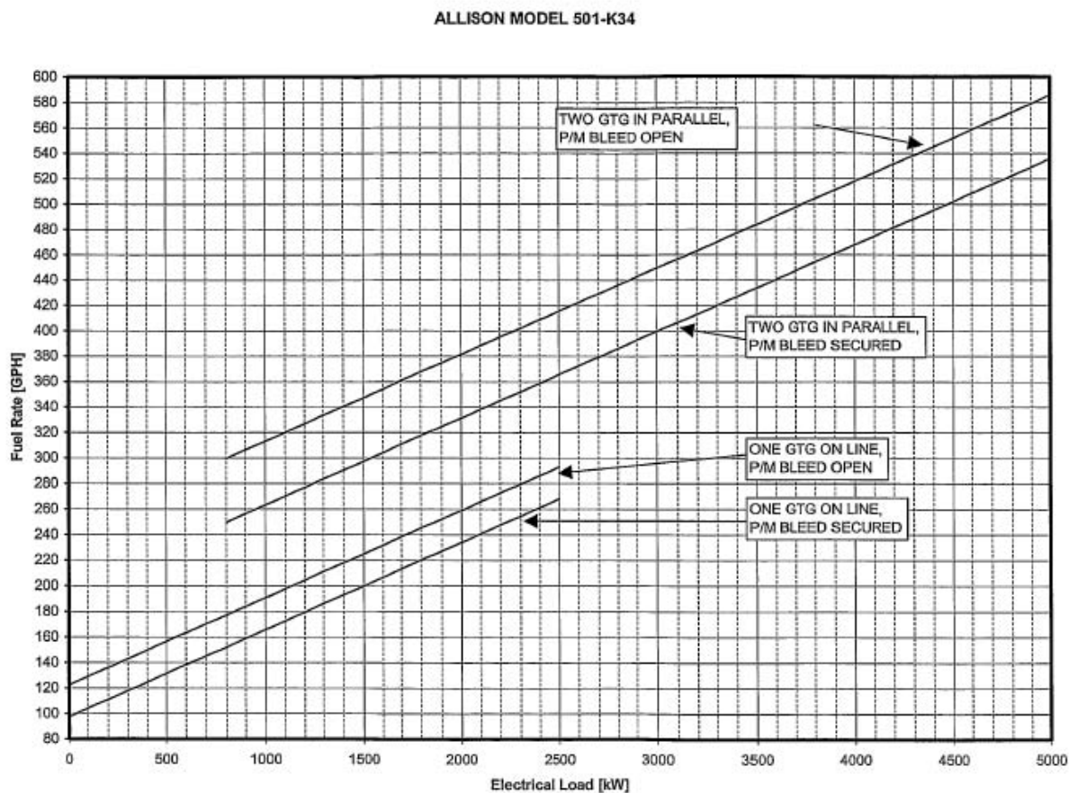
DDG 51 CLASS FUEL RATE NOMOGRAM
