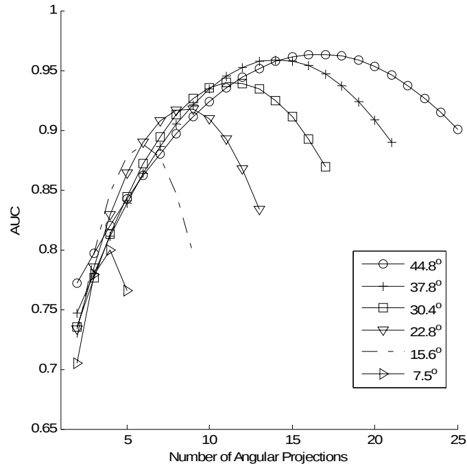
Fig. 10: Variation of AUC with the number of projections for projection images (a) and reconstructed slices (b) under iso-study dose conditions at different angular ranges in 7.5^\circ - 45^\circ range. The total dose level was fixed to that of single-view mammography.
