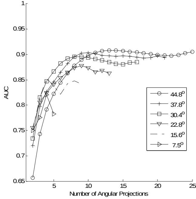
Fig. 7: Variation of AUC with number of projections for CI (a) and tomosynthesis (b), at different acquisition dose levels under iso-image dose condition (dose of each projection was fixed at 1/25 th fraction of typical single-view mammography). The angular spans of these projections were in the 7.5° – 45° range.
