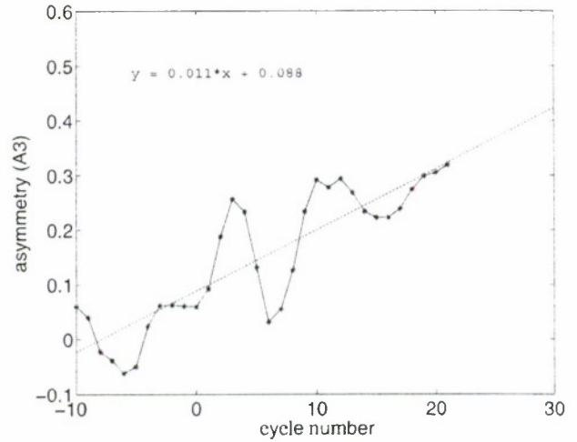
Fig. 2. Similar to Fig. 1, here presented for the smoothed values A_3 .
