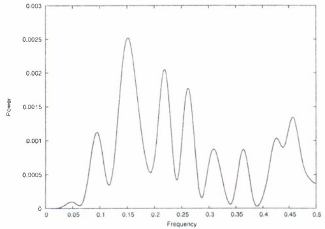
Fig. 3. The power spectrum as a function of the inverse cycle number for the data series presented in Fig. 1. The highest peak corresponds to the period of about 70 years.
