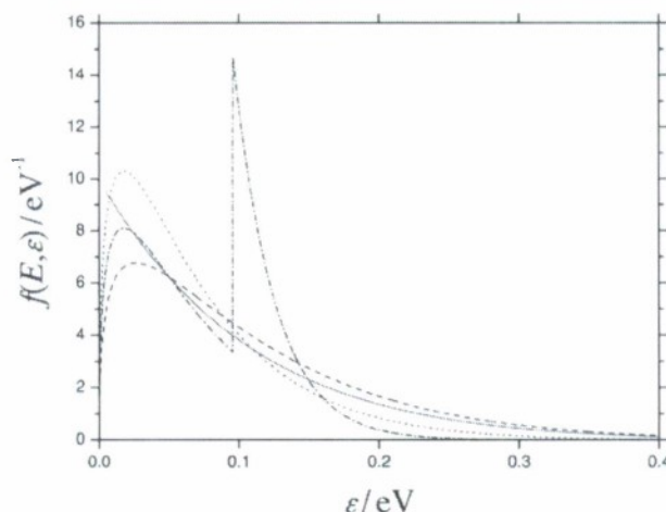
FIG. 3. Energy distribution f(E, \epsilon) of electrons from the detachment from \text{SF}_6^- ( E - EA = 1 eV); full line: RRKM-type model; dashed line: electron capture VW model; dotted line: electron capture with IVR model; dash-dotted line with peak near 0.1 eV: electron capture with IVR and VEX model, see text.
