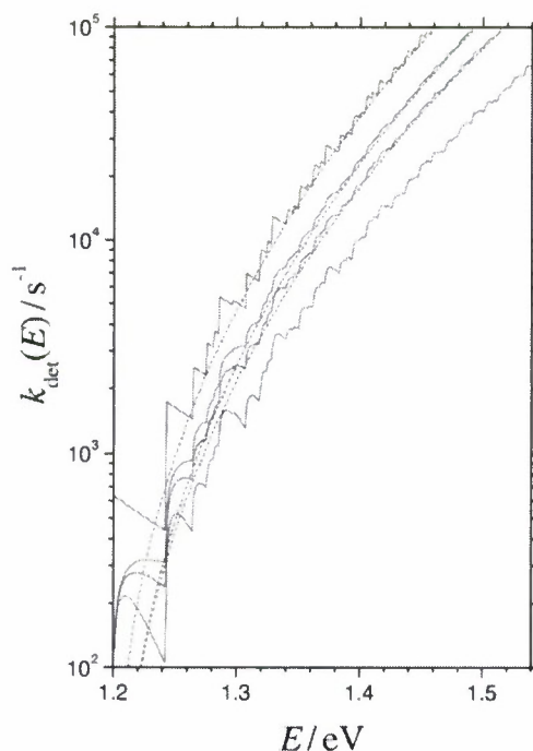
FIG. 2. Specific rate constants k_{\text{det}}(E) for electron detachment from \text{SF}_6^- . Curves from top to bottom: (i) RRKM-type model without electron capture contributions, i.e., P(E-E_{0i})=1 for E>E_{0i} ; (ii) pure electron capture model, i.e., P(E-E_{0i})=P^{\text{VW}}(E-E_{0i}) ; (iii) electron capture with IVR contribution, i.e., P(E-E_{0i})=P^{\text{VW}}(E-E_{0i})P^{\text{IVR}}(E-E_{0i}) ; (iv) electron capture with IVR and VEX contributions, i.e., P(E-E_{0i})=P^{\text{VW}}(E-E_{0i})P^{\text{IVR}}(E-E_{0i})P^{\text{VEX}}(E-E_{0i}) . Full curves: Detailed calculations from Ref. 15; dashed curves for the upper three models: Simplified calculations with Eq. (3.9) from the present work, see text.
