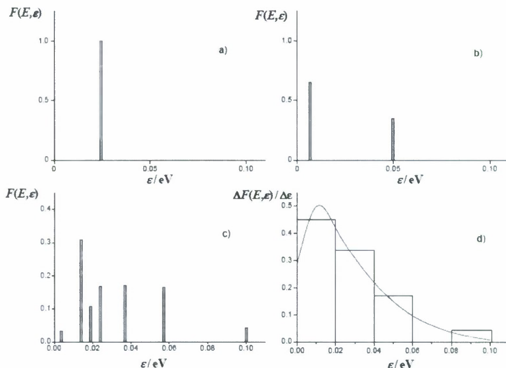
FIG. 1. Discrete distributions F(E, \epsilon) of electron energies \epsilon in the detachment from SF 6 - at the energies E - EA = 0.025 eV (a), 0.05 eV (b), and 0.1 eV [(c) and (d)]. (d) shows \Delta F(E, \epsilon)/\Delta \epsilon with bins \Delta \epsilon = 0.02 eV; the continuous curve is from Eq. (2.12), see text.
