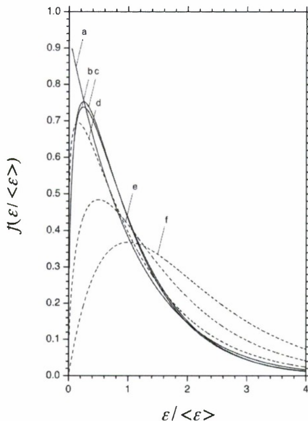
FIG. 4. Energy distribution f(E, \epsilon(E)) of electrons from the detachment from \text{SF}_6^- ( E - \text{EA} = 1 eV); full curves=detailed calculations: (a) RRKM-type model with \langle \epsilon \rangle = 0.0937 eV, (b) electron capture VW-model with \langle \epsilon \rangle = 0.109 eV, and (c) VW+IVR-model with \langle \epsilon \rangle = 0.0730 eV; dashed curves=model functions (3.10) with exponents n=0.15 (d), 0.5 (e), and 1.0 (f).
