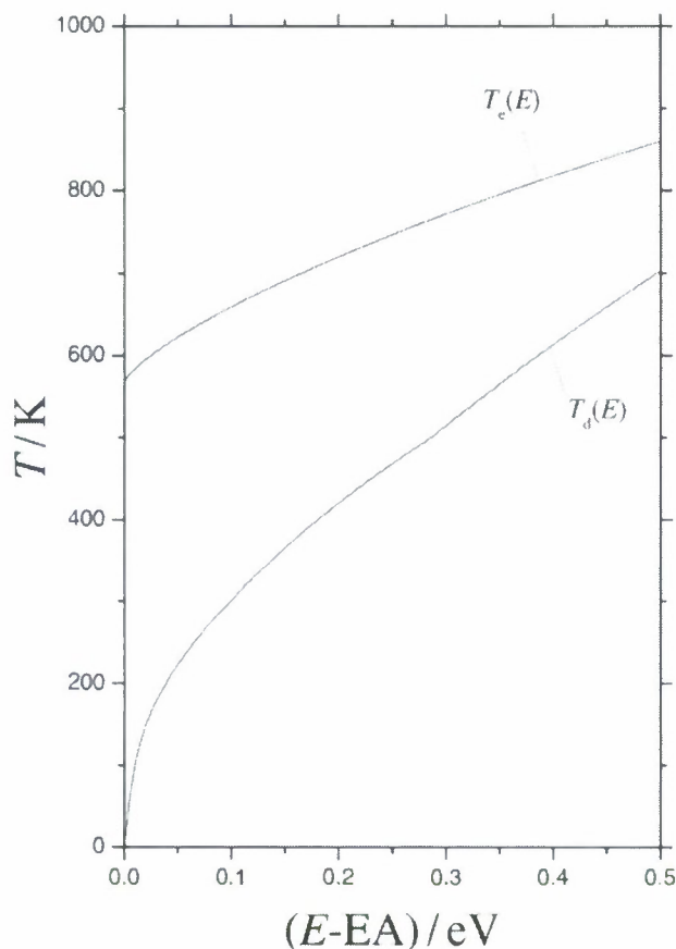
FIG. 7. Comparison of the daughter temperature T_d(E) , based on Eq. (4.1), and an effective or isokinetic temperature T_e(E) , from Eq. (4.9), in thermionic emission models of electron detachment from \text{SF}_6^- (detailed calculations of this work, see text).
