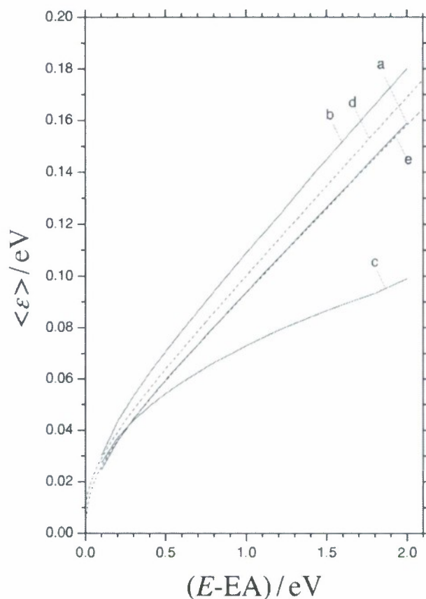
FIG. 5. Average energy \langle \epsilon \rangle of electrons detached from \text{SF}_6^- at total energy E . Full curves=detailed calculations; (a) RRKM-type model; (b) electron capture VW-model; (c) electron capture with IVR=VW+IVR model. Dashed lines=thermionic emission results; (d) putting \langle \epsilon \rangle = 0 in Eq. (4.1); (e) including finite \langle \epsilon \rangle from Eqs. (4.1), (4.2), and (4.4); see text.
