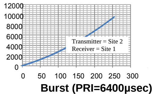
Figure 4.18: Multi-Static Modeled Phase Errors
