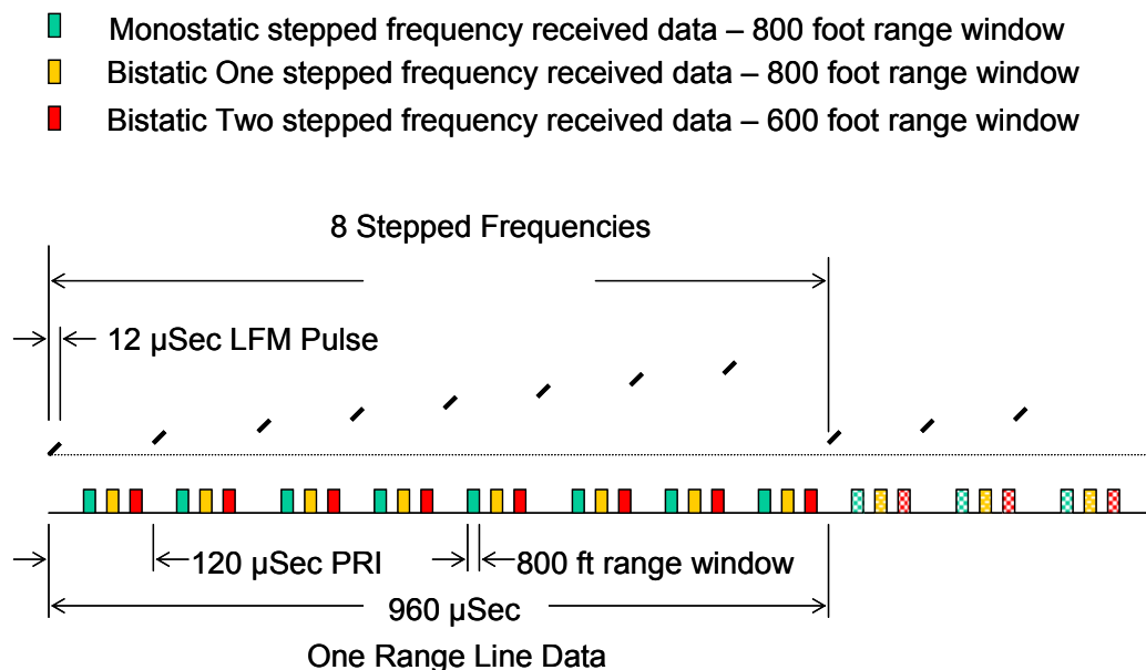
Figure 4.13: Multi-static ISAR Received Signal Data – Chirp Processed
