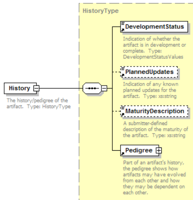
Figure 37. History Element
