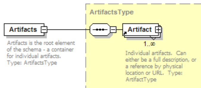
Figure 23. Artifacts Element
