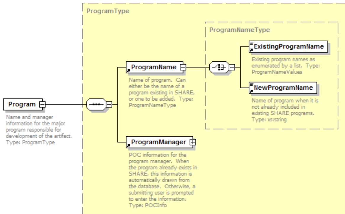
Figure 30. Program Element
