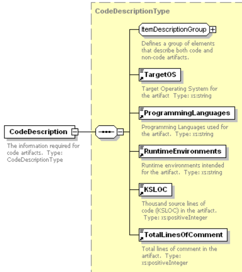
Figure 40. CodeDescription Element
