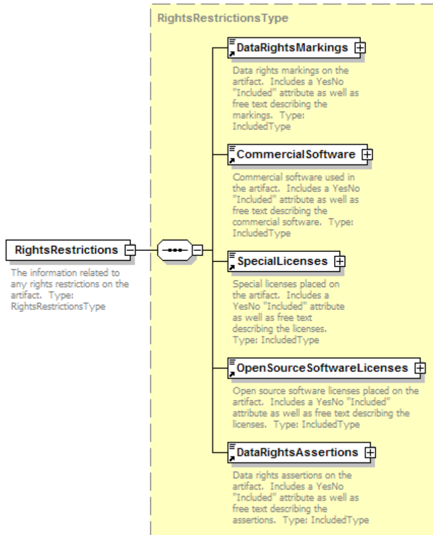
Figure 45. RightsRestrictions Element
