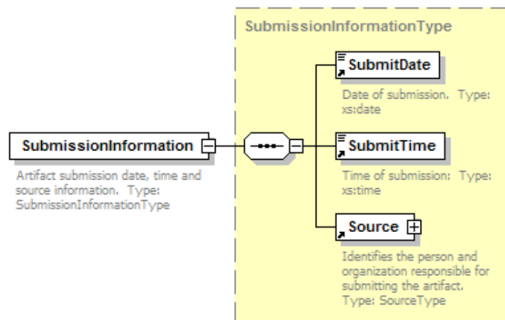
Figure 26. SubmissionInformation Element
