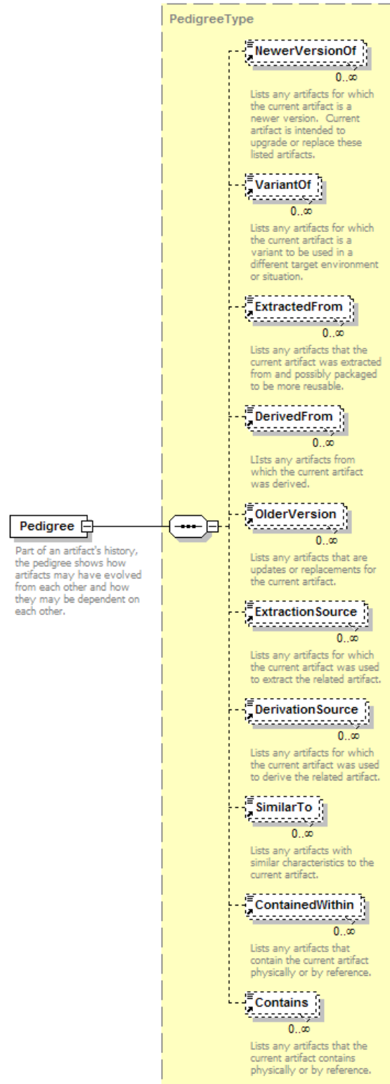
Figure 38. Pedigree Element
