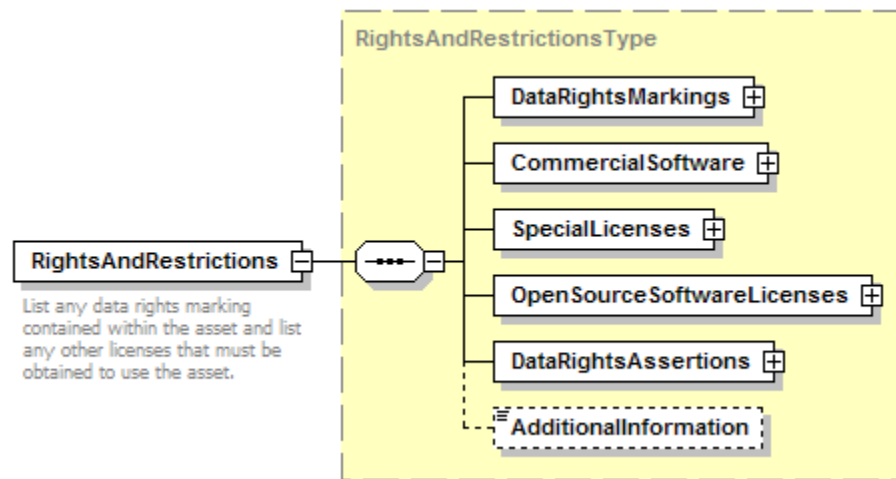
Figure 22. RightsAndRestrictions Element
