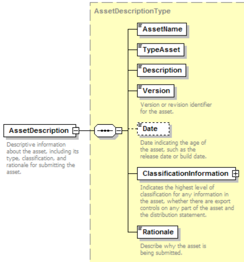
Figure 9. AssetDescription Element
