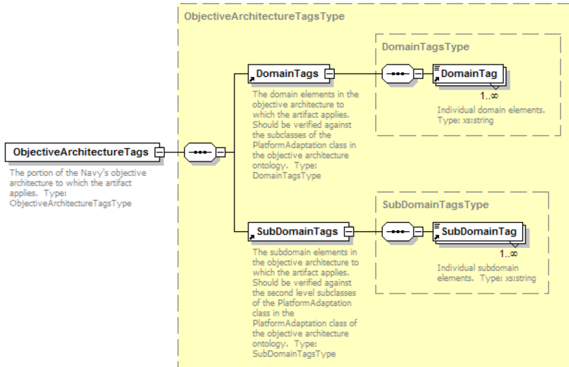
Figure 35. ObjectiveArchitectureTags Element
