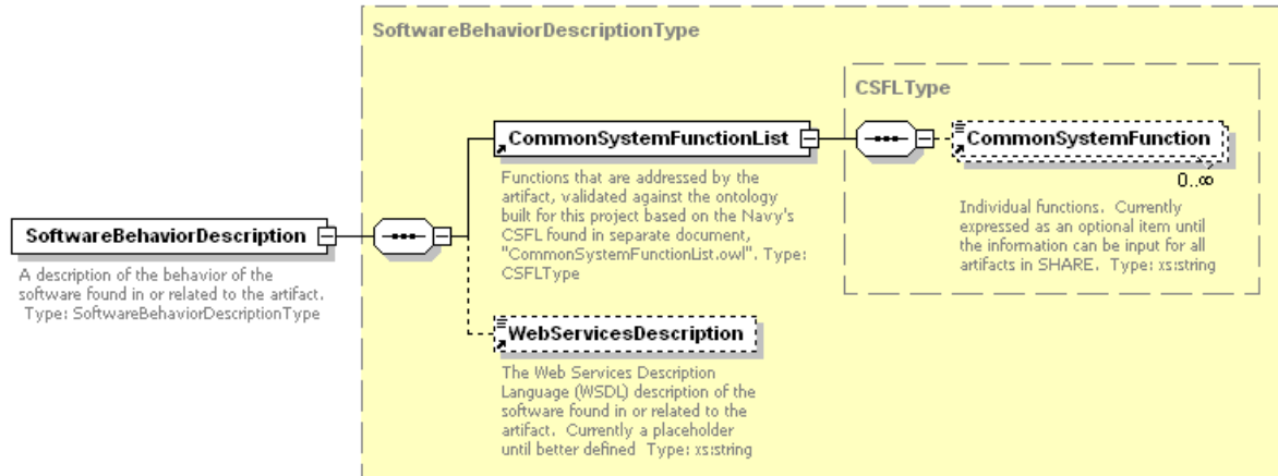
Figure 36. SoftwareBehaviorDescription Element
