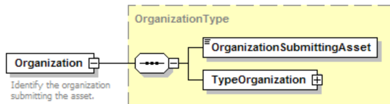
Figure 4. Organization Element
