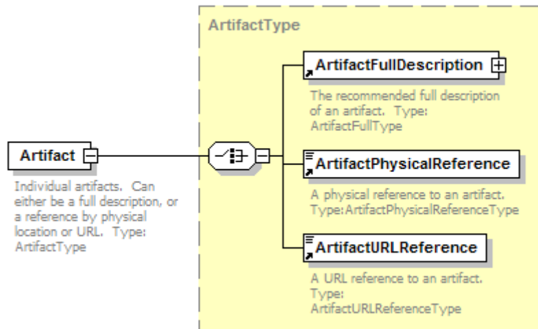
Figure 24. Artifact Element
