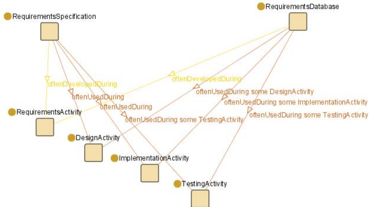
Figure 55. Properties Assigned to RequirementsSpecification and RequirementsDatabase Classes
