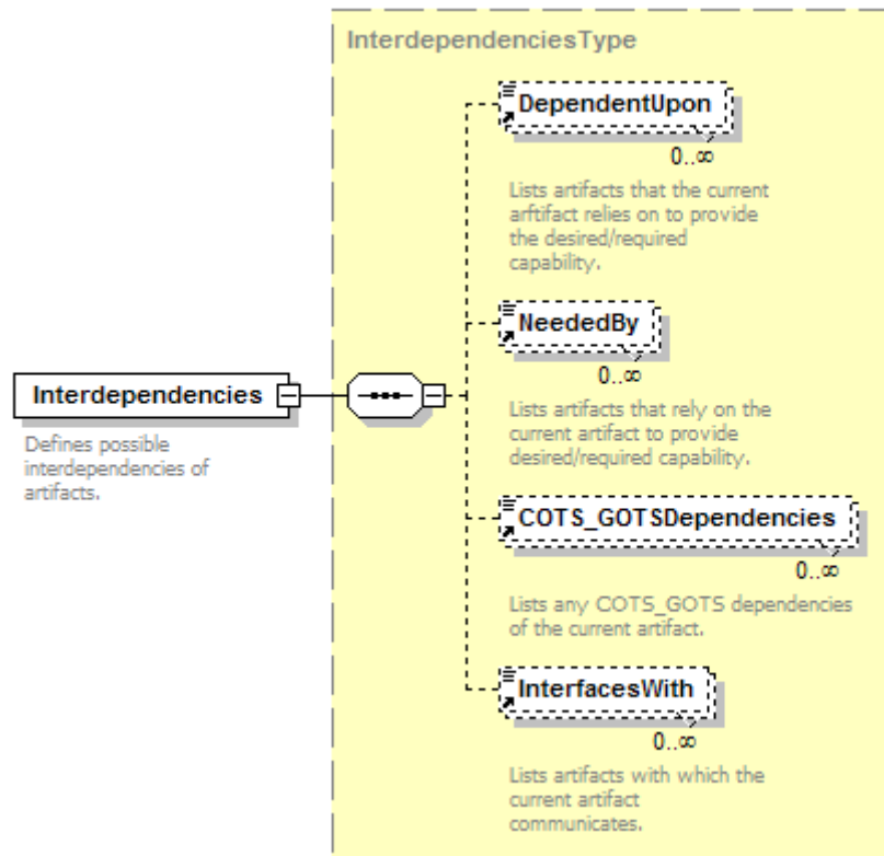
Figure 39. Interdependencies Element
