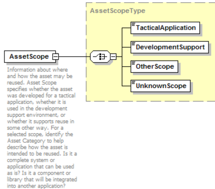
Figure 11. AssetScope Element
