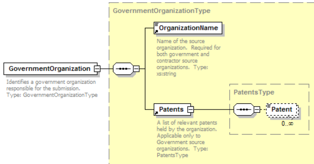
Figure 28. GovernmentOrganization Element
