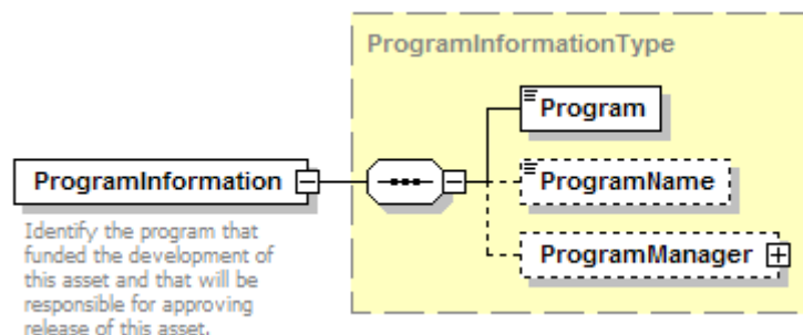
Figure 8. ProgramInformation Element
