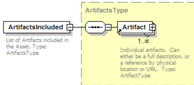
Figure 49. ArtifactsIncluded Element
