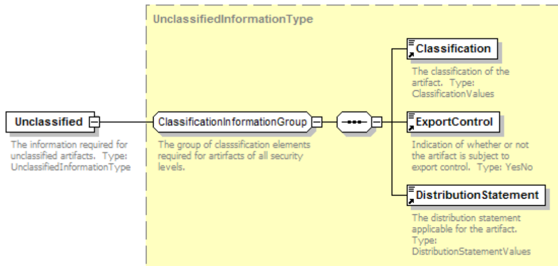
Figure 42. Unclassified Element
