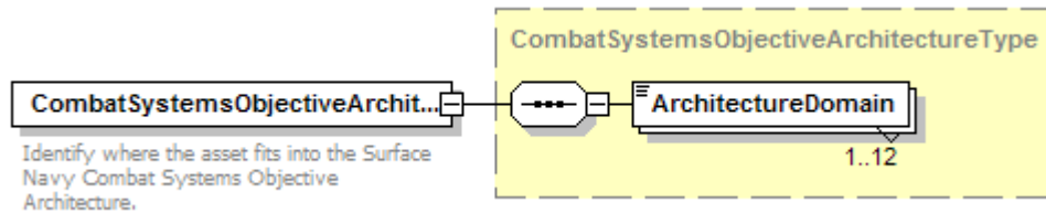
Figure 20. CombatSystemsObjectiveArchitecture Element
