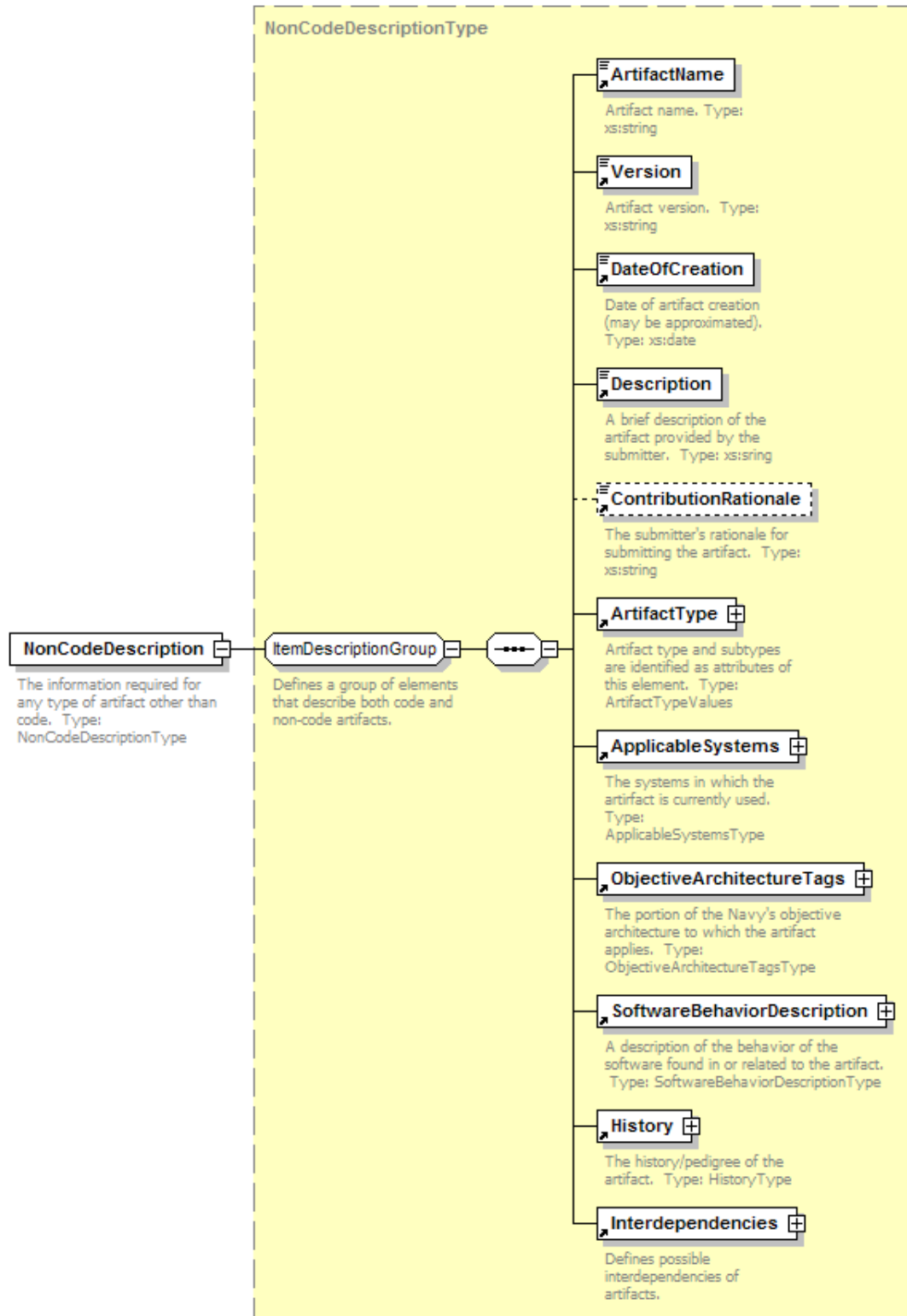
Figure 32. NonCodeDescription Element
