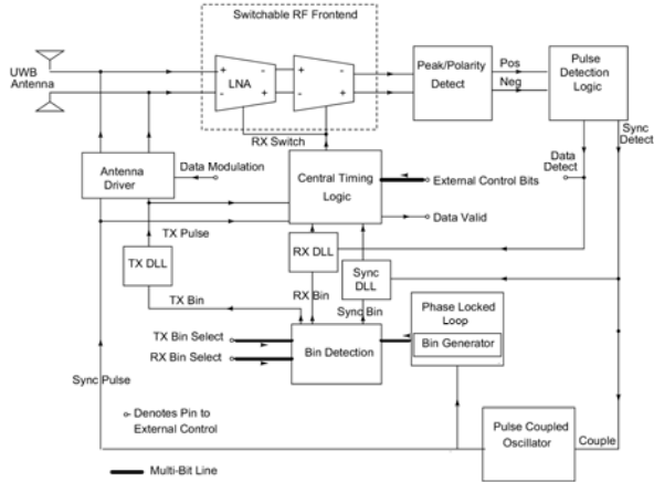
Figure 9 General Transceiver Node
