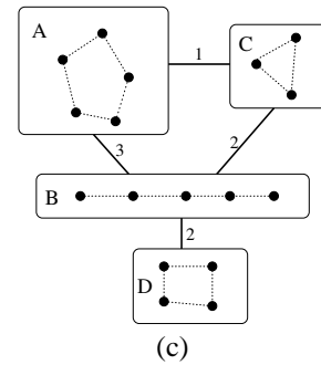
Figure 8: Explicit representation and aggregation of spatial adjacencies. (a) Neighborhood graph edges are classified into strong (solid) and weak (dashed) adjacencies. (b) Strong adjacencies connect internal structure of aggregate objects A, B, and C. (c) A higher-level neighborhood graph is constructed from lower-level weak adjacencies between constituent objects.
