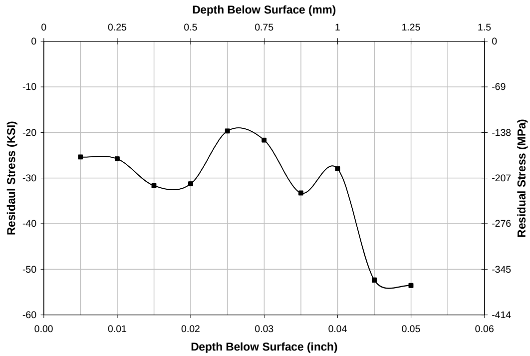
Figure 2. Residual stress profile of case-carburized M50NiL
