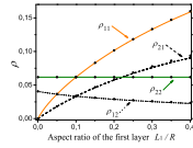
Figure 2. (Color online) The dimensionless dipolar parameters \rho_{jk} , which define the self- and cross-demagnetization tensors for the system of two thin disks coupled by dipole-dipole interaction, as functions of the aspect ratio of the first disk L_1/R . The aspect ratio of the second disk and the distance between the disks are fixed: L_2/R = 1/10 , d/R = 1/25 . Solid, dashed, and dotted lines were calculated from the approximate analytical expressions (12) and (13). Dots were obtained from the exact expressions (9) and (10).
