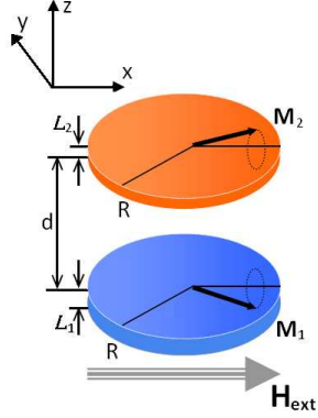
Figure 1. (Color online) Nano-pillar with two ferromagnetic layers coupled by the dipole-dipole interaction in constant bias magnetic field \mathbf{H}_{ext} , directed along the x -axes. Thicknesses of the layers L_{1,2} and the distance d between them are much smaller than the layers radii R . The layers have the same saturation magnetization M_1 = M_2 = M ( 4\pi M = 8 kOe, which is typical for permalloy).
