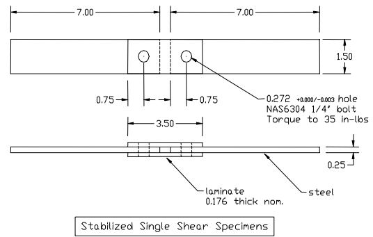
Figure 7. Boeing Stabilized Single Lap-Shear Test
