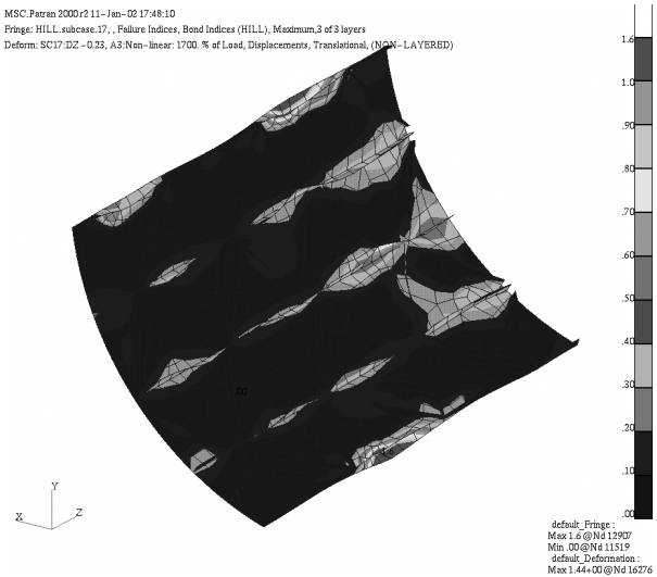
Figure 19. Optimized Panel, 2-tows Axial Stiffeners, Hill Failure Index
