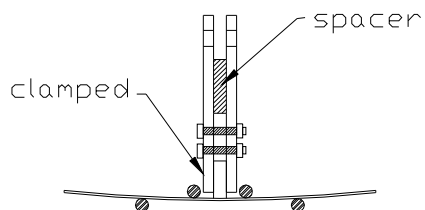
Figure 4. Pull-off Tee Test Fixture Detail
