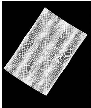
Figure 14. Minimum Principal Stress (Axial Skin Stresses)
