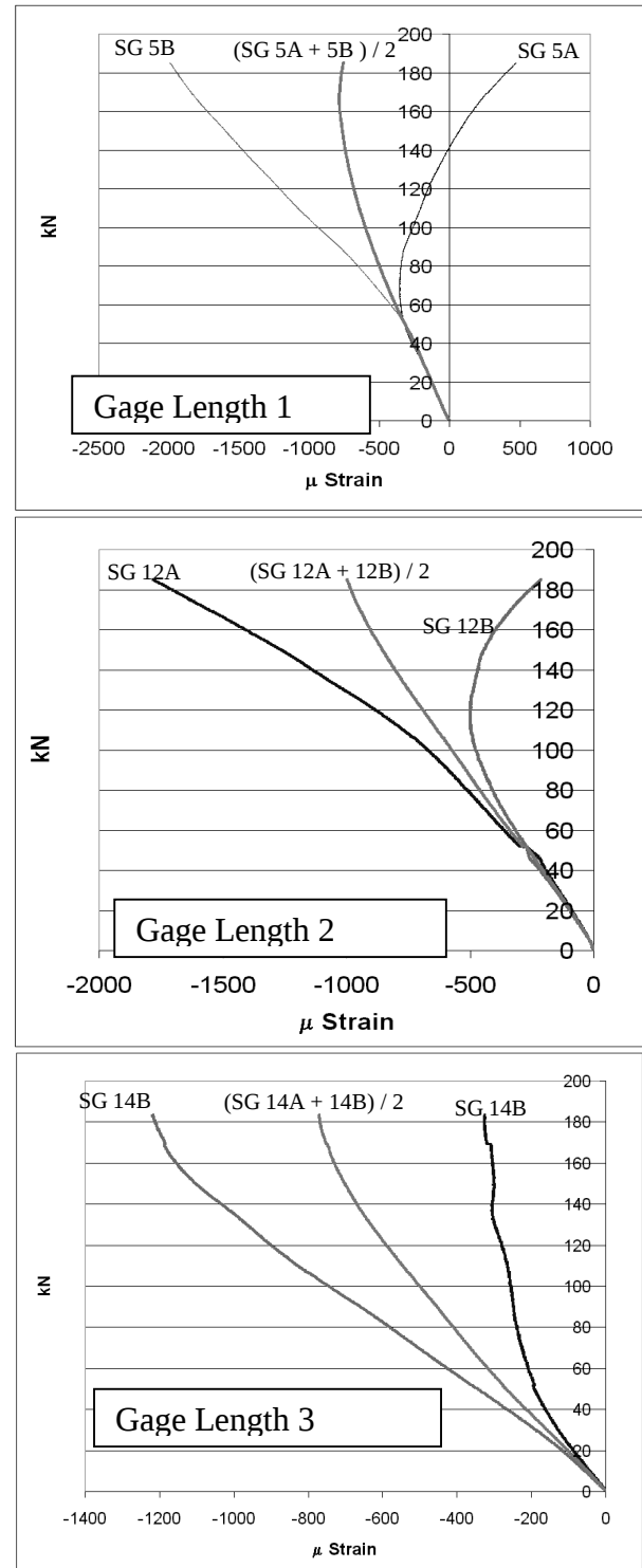
Figure 12. Axial Strains at Points along Axial Rib Gage Lengths 1, 2, and 3.
