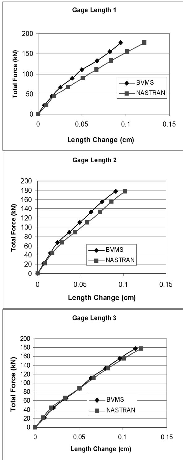
Figure 11. Comparison of BVMS Measured and AFRL Calculated Axial Rib Response.
