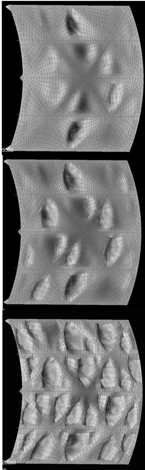
Figure 5. Progression of Skin Pocket Buckling Response of Baseline Panel at Total Panel Loads of 60,309 N, 79,370 N, and 189,326 N (Collier 2002)
