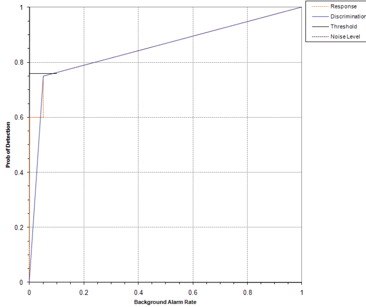
Figure 3. Dual Mode SAM/towed blind grid probability of detection for response and discrimination stages versus their respective probability of background alarm over all ordnance categories combined.
