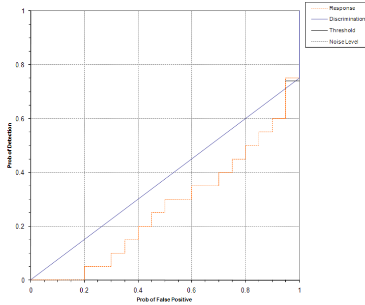
Figure 4. Dual Mode SAM/towed blind grid probability of detection for response and discrimination stages versus their respective probability of false positive for all ordnance larger than 20 mm.
