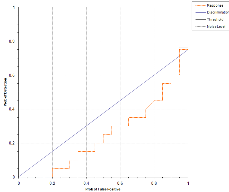
Figure 2. Dual Mode SAM/towed blind grid probability of detection for response and discrimination stages versus their respective probability of false positive over all ordnance categories combined.
