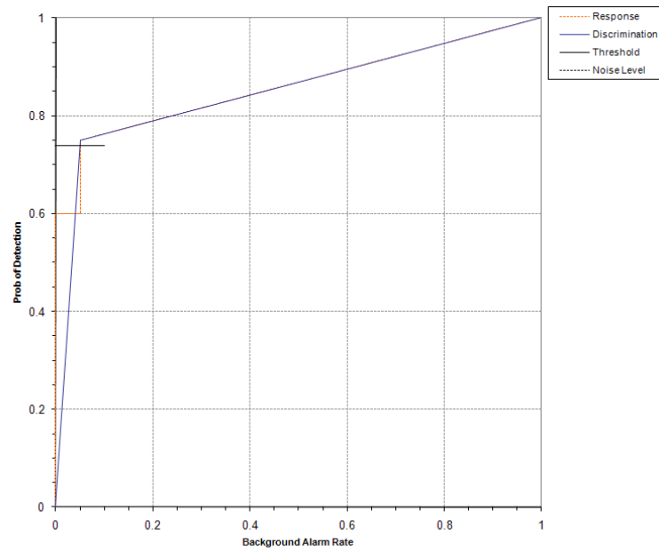
Figure 5. Dual Mode SAM/towed blind grid probability of detection for response and discrimination stages versus their respective probabilities of background alarm for all ordnance larger than 20 mm.
