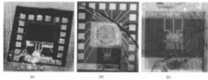
Fig. 2. Fully integrated MCM. (a) Top view showing CLDA and VCSEL array. (b) Bottom view of CLDA and VCSEL array as seen through lenslet array. (c) Close-up of lenslet array beneath the VCSEL.
