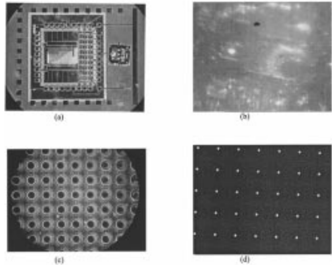
Fig. 3. Demonstration of VCSEL fan-out. (a) CLDA integrated with 1 \times 3 VCSEL array. (b) Lasing of multimode 850\text{-nm} VCSEL. (c) Diffractive lenslet array. (d) Image of 5 \times 7 array of focussed spots generated 160\text{ mm} from DOE surface.
