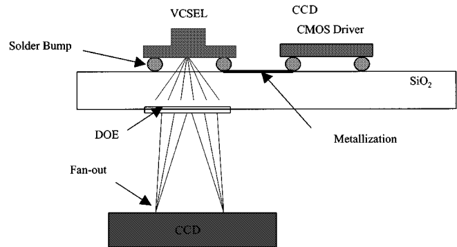
Fig. 1. Schematic representation of optoelectronic multichip module.
