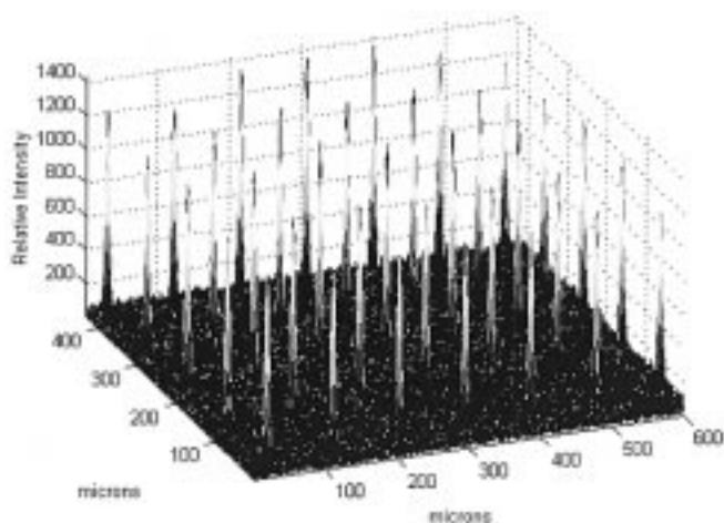
Fig. 4. Intensity plot of the focal spots in the image plane.
