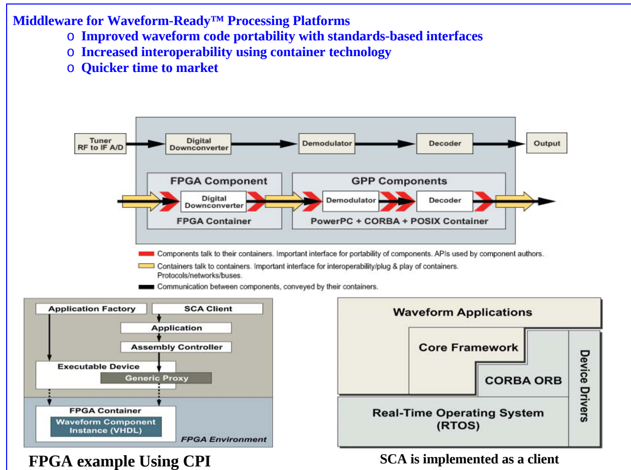
Figure 2: CPI Data Flow Model
