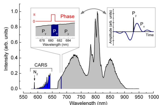
FIG. 1. (Color online) Spectrum of the 7 fs laser beam and the CARS signal. In the left inset, the phase and polarization masks are shown; P_x and P_y correspond to orthogonal polarizations. In the right inset, the temporal profiles of the excitation and probe parts of the beam are shown along with their overlap.
