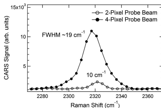
FIG. 2. Room temperature CARS spectra of \text{N}_2 for two spectral bandwidths of the probe pulse.
