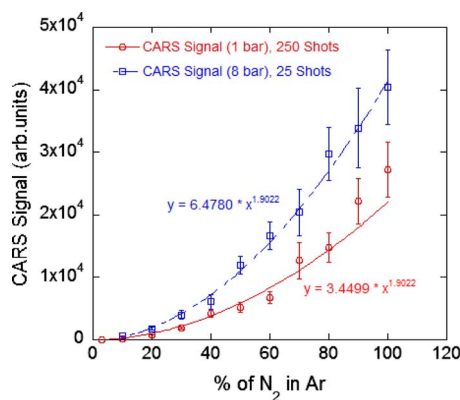
FIG. 4. (Color online) Femtosecond-CARS signal of gas-phase N_2 in mixtures with Ar at total cell pressures of one bar and eight bar. The solid and dashed lines represent the power curves fit through the data points.
