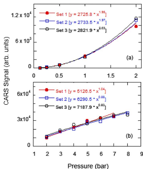
FIG. 3. (Color online) Single-beam femtosecond-CARS signal as a function of pressure. Symbols represent experimental data points; solid lines represent power curves fit through the data points. Three sets of data are shown to illustrate the repeatability of the observed signal dependence on the number density of N_2 .
