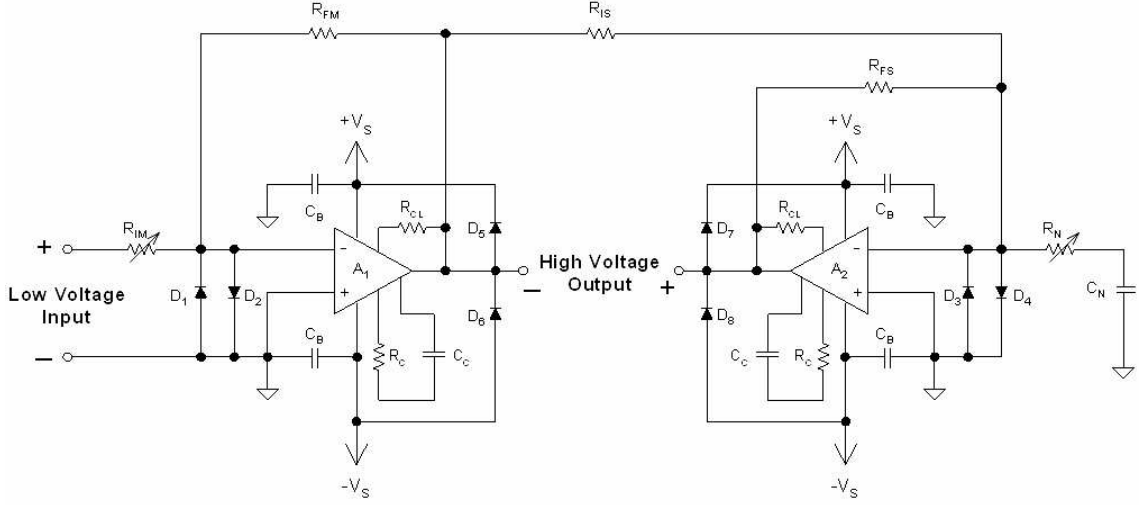
Figure 4.6: Schematic of the high-voltage amplifier section
