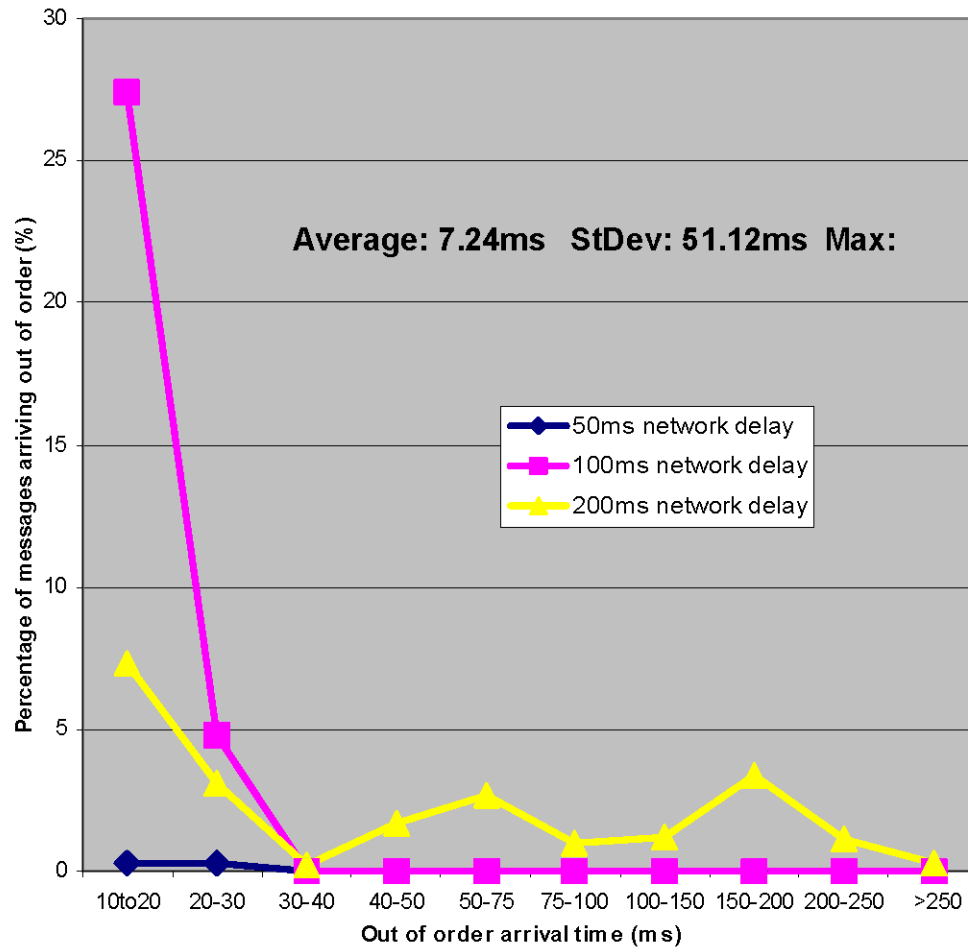
Figure 2-8 Message Arrival on WAN: Graph 6
