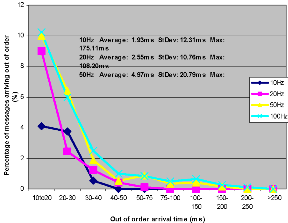
Figure 2-3 Message Arrival on WAN: Graph 1
