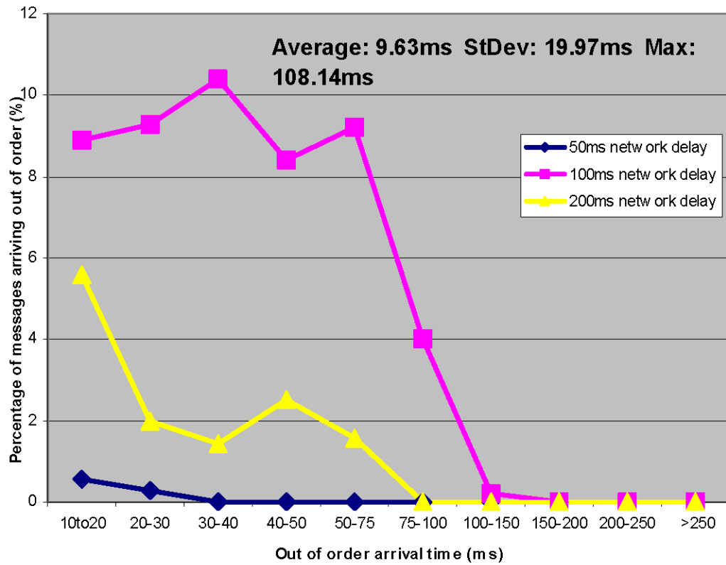
Figure 2-6 Message Arrival on WAN: Graph 4
