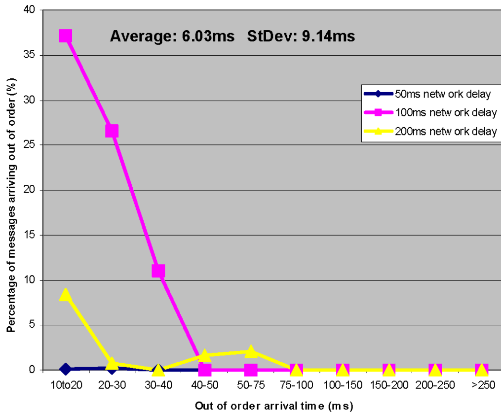
Figure 2-7 Message Arrival on WAN: Graph 5
