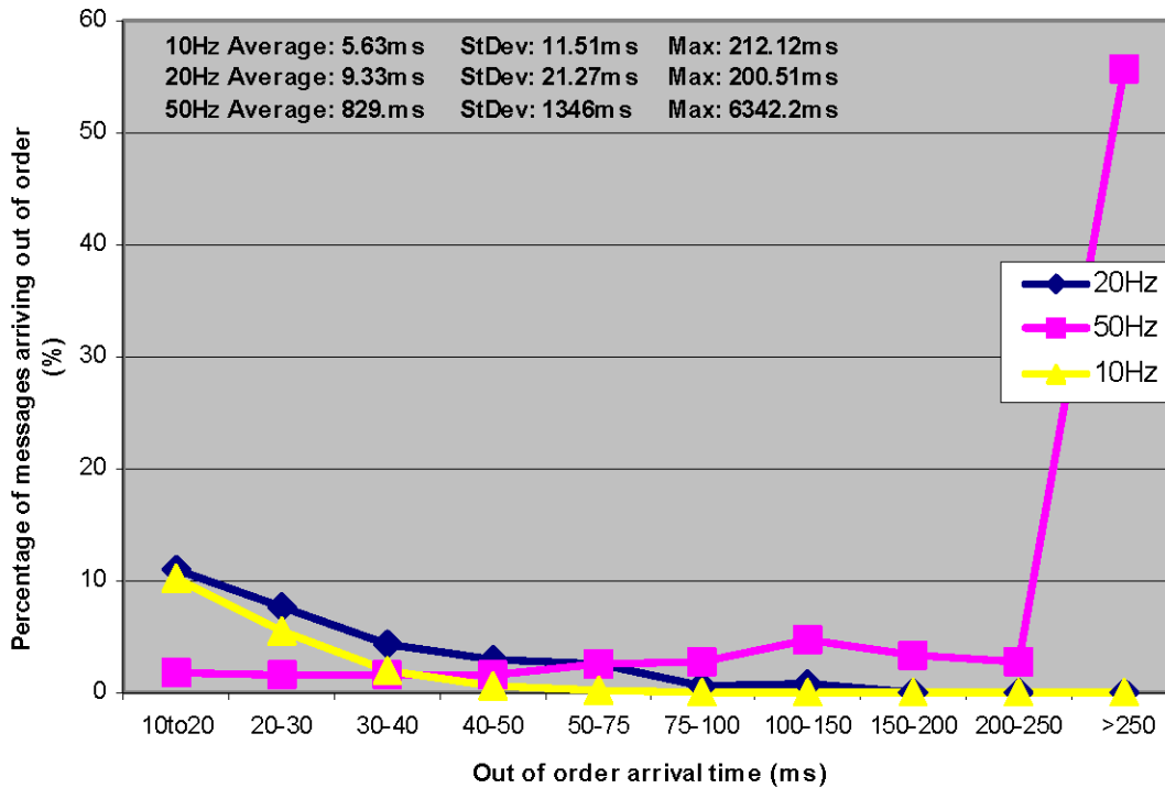
Figure 2-5 Message Arrival on WAN: Graph 3
