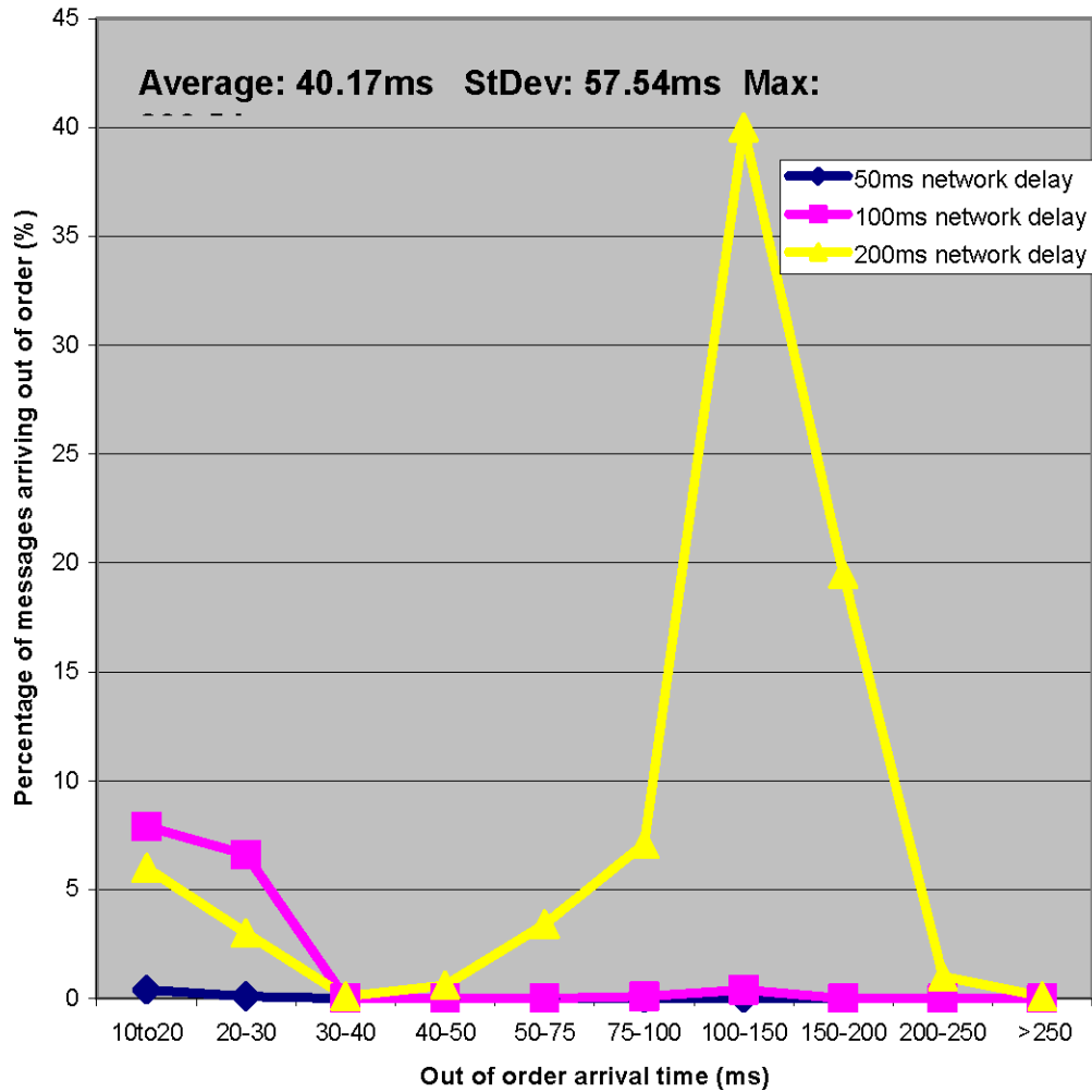
Figure 2-9 Message Arrival on WAN: Graph 7
