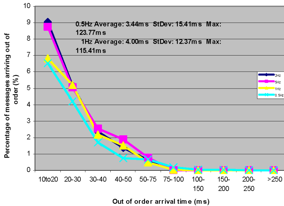
Figure 2-4 Message Arrival on WAN: Graph 2
