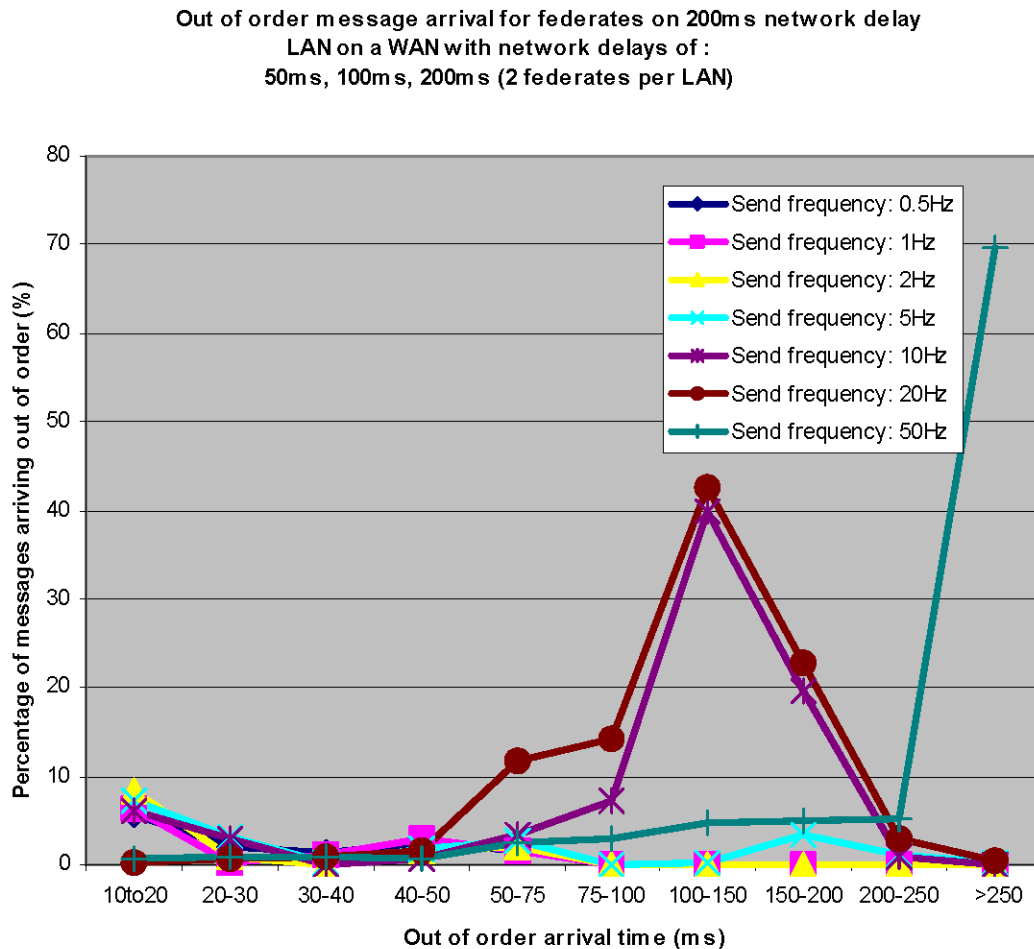
Figure 2-13 Message Arrival on WAN: Graph 9
