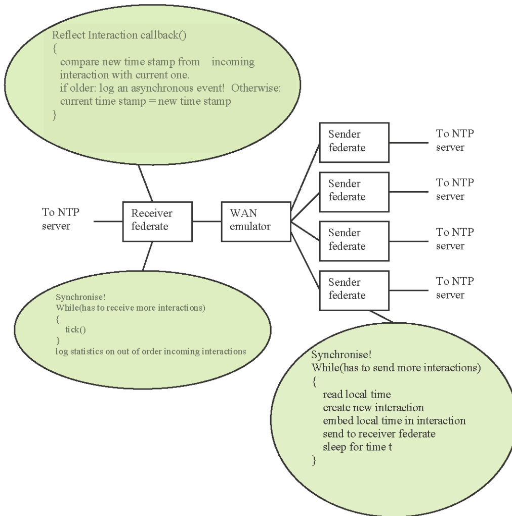
Figure 2-1 A Non-Time-Managed Federation
