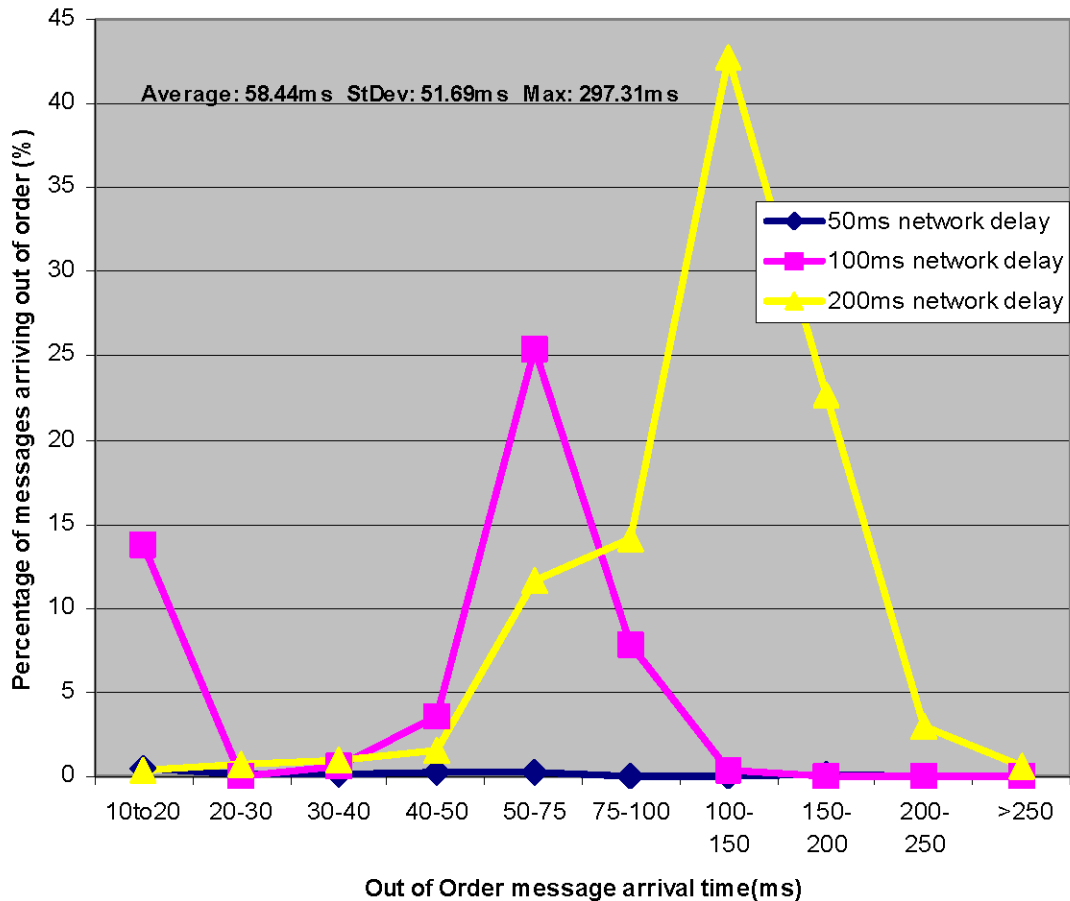
Figure 2-10 Message Arrival on WAN: Graph 8
