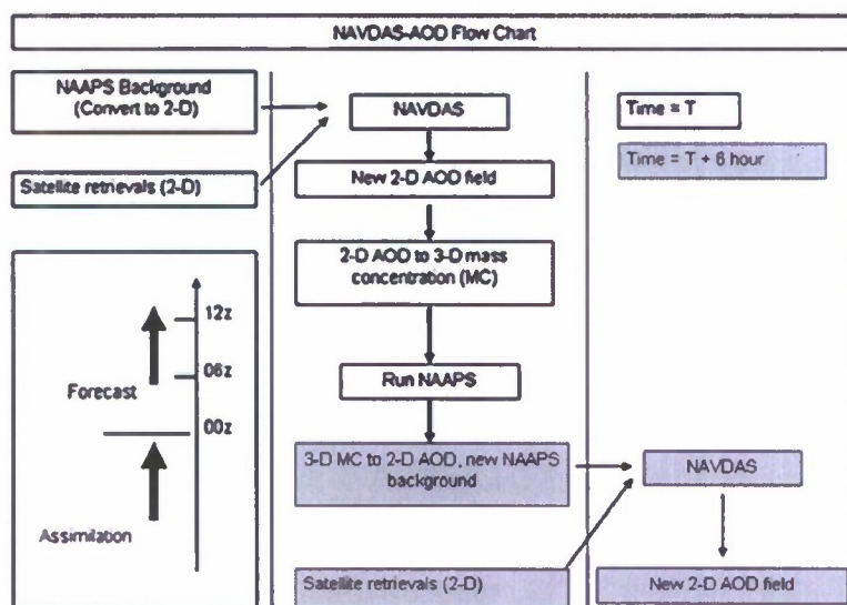
Figure 1. Flowchart of the NAVDAS-AOD.
