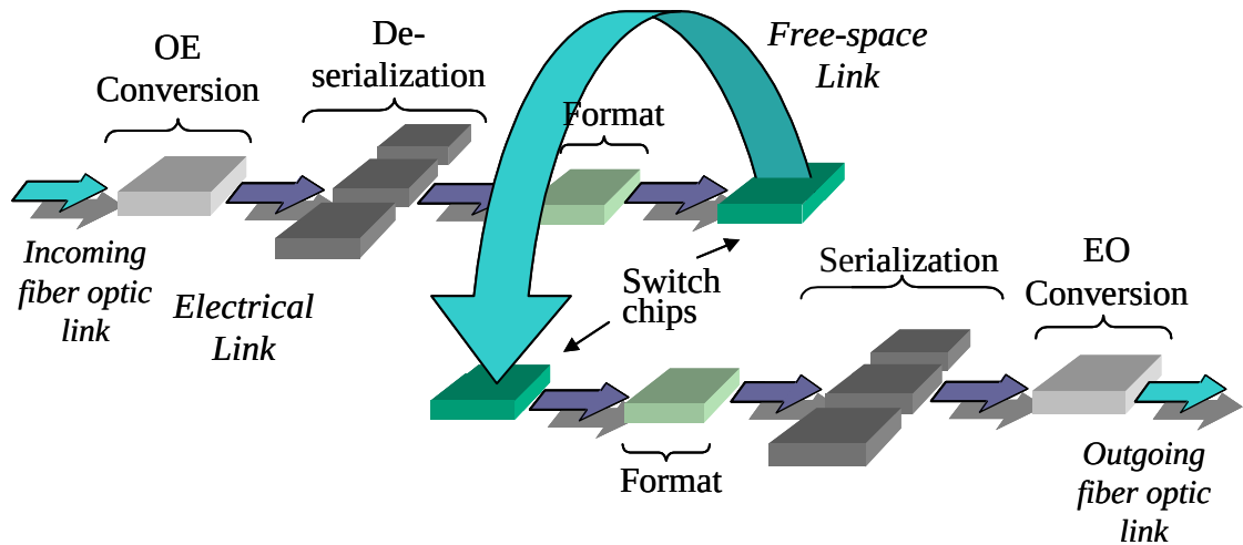
Figure 1. Dataflow through switch (one path, one direction shown).
