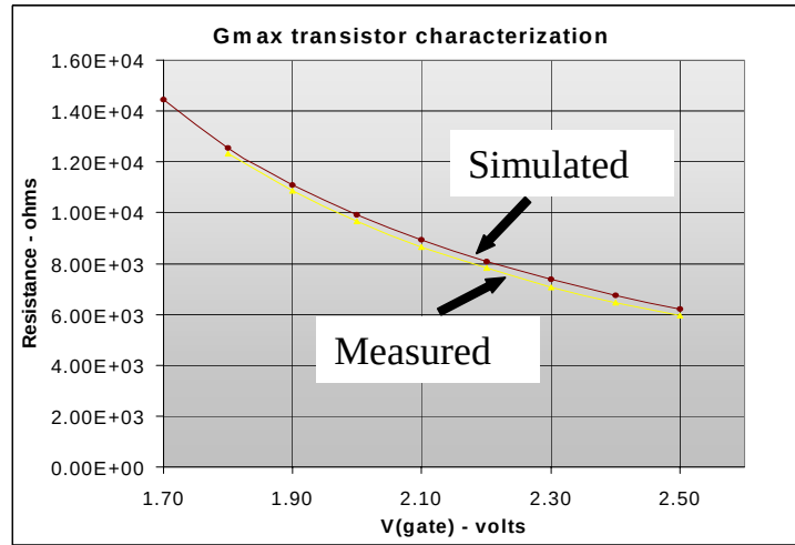
Figure 27. Test and simulation data showing DC characteristic of one of the feedback transistors within the receiver pre-amplifier. Good correlation is observed.
