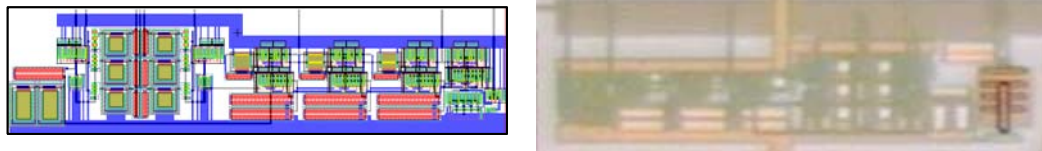
Figure 20. Receiver cell. (left) Layout. (right) Microphotograph of fabricated circuit.
