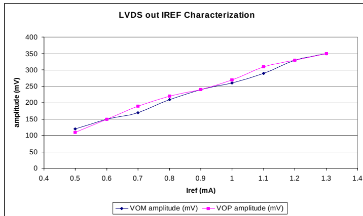
Figure 24. Test data from electrical characterization of the Test ASIC LVDS Output driver. The I_{ref} input being swept controls the bias voltage of the CML buffer stages and LVDS output stage of the LVDS driver.
