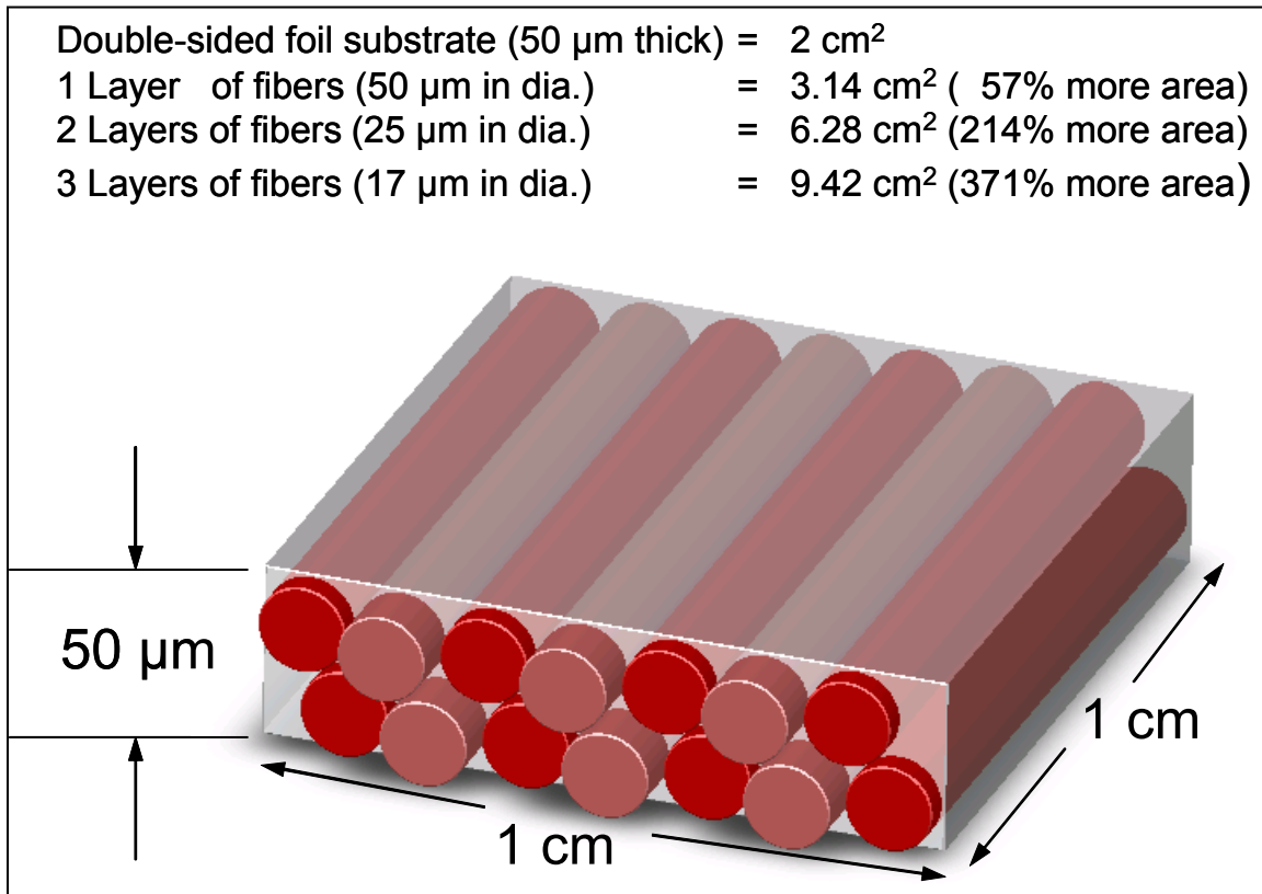
Figure 11: Comparison between the useable battery area of a flat 50 \mu\text{m} thick foil substrate (commonly used by ITN for the fabrication of flat thin-film batteries) and a PowerFiber array of the same footprint and overall volume. Note that thin-film batteries can practically not be fabricated on the edge of such a foil substrate so that only both face sheet surfaces ( 2 \times 1 \text{ cm}^2 = 2 \text{ cm}^2 ) are available.
