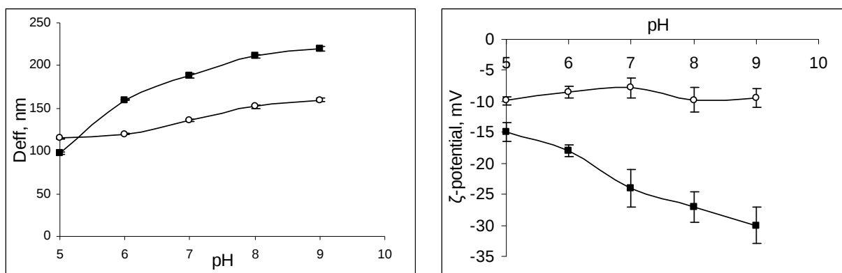
Figure 2. Physicochemical characteristics of c /PEO- b -PMA nanogels (■) and IgG- c /PEO- b -PMA (○): effective diameter ( D_{eff} ) and \zeta -potential of nanogels with 20% targeted degree of cross-linking as a function of pH.
