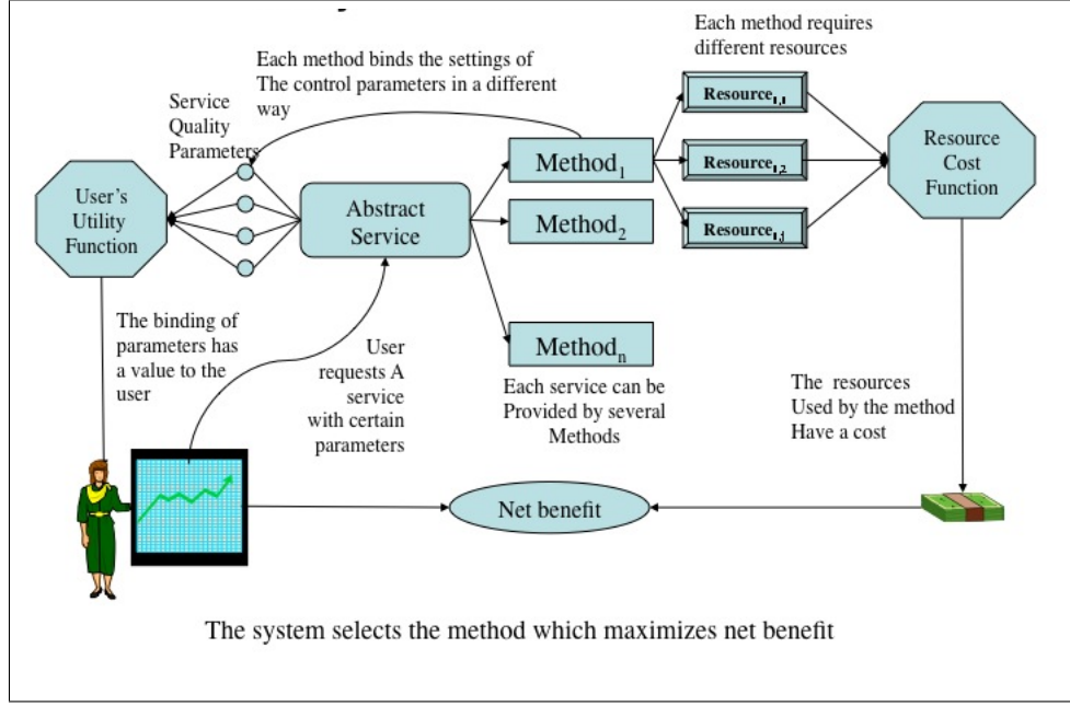
Figure 43: Adaptive Software
