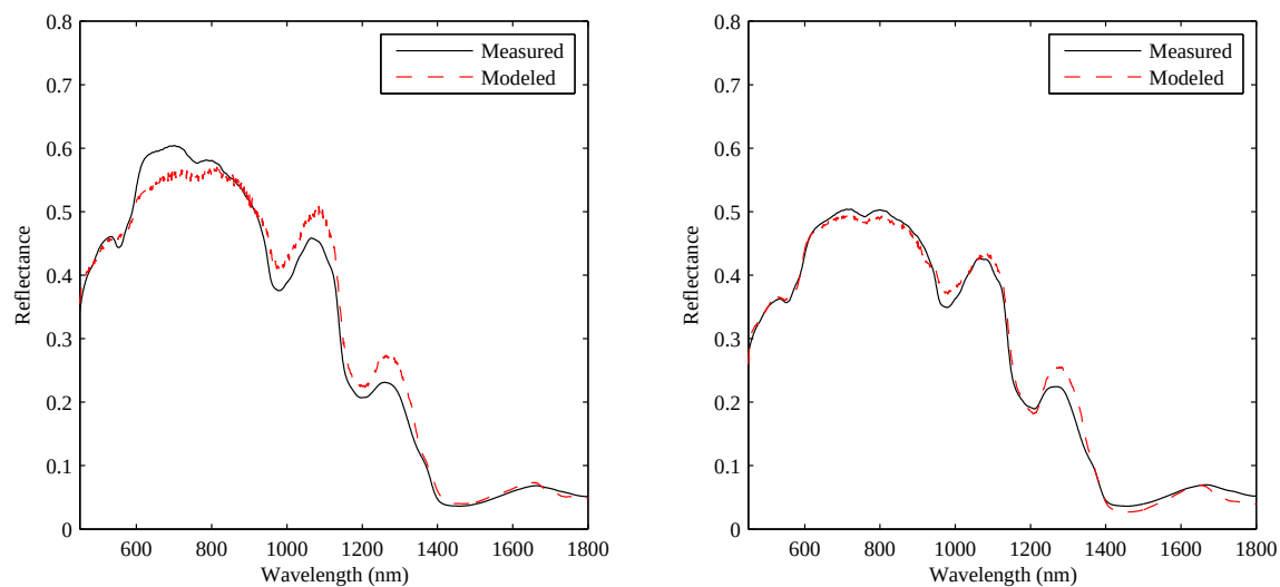
Figure 107: Comparison of model and measured cadaver skin reflectance for sample 45 and 46.
