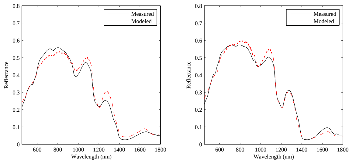
Figure 109: Comparison of model and measured cadaver skin reflectance for sample 49 and 50.
