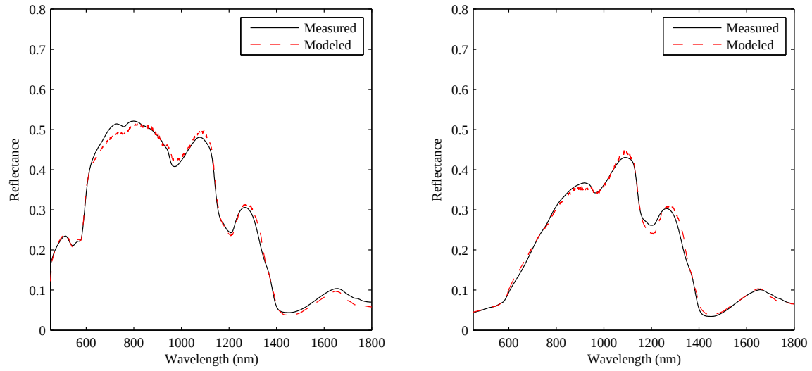
Figure 95: Comparison of model and measured living skin reflectance for sample 21 and 22.
