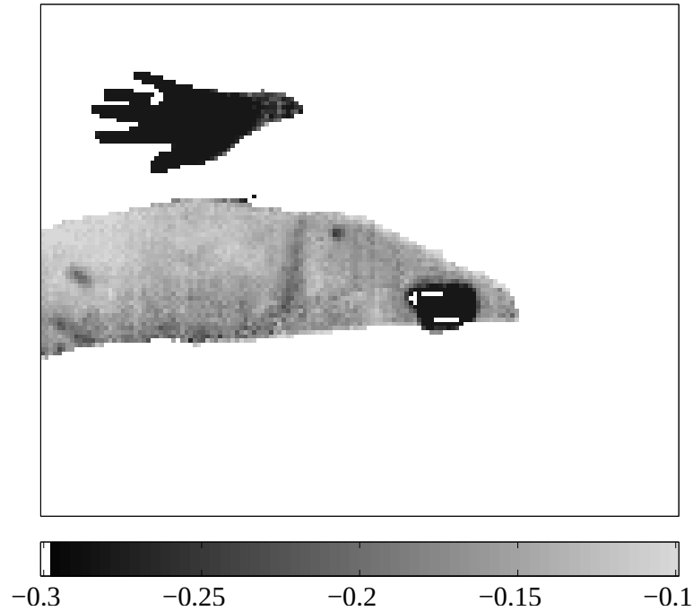
Figure 77: NDGRI values of the fair-skinned cadaver and the palm of the living person in Fig. 76.
