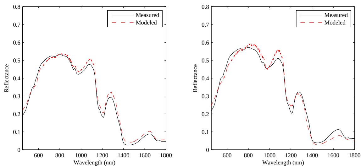
Figure 110: Comparison of model and measured cadaver skin reflectance for sample 51 and 52.
