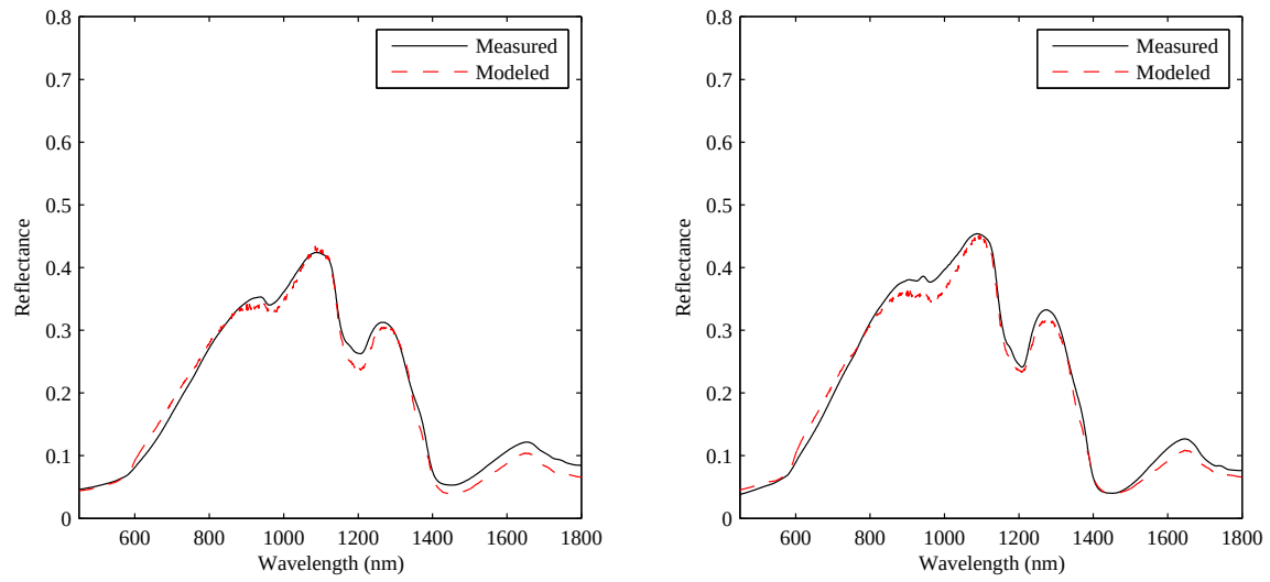
Figure 92: Comparison of model and measured living skin reflectance for sample 15 and 16.
