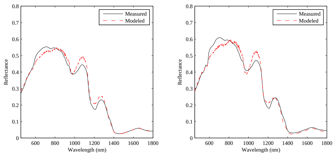
Figure 102: Comparison of model and measured cadaver skin reflectance for sample 35 and 36.
