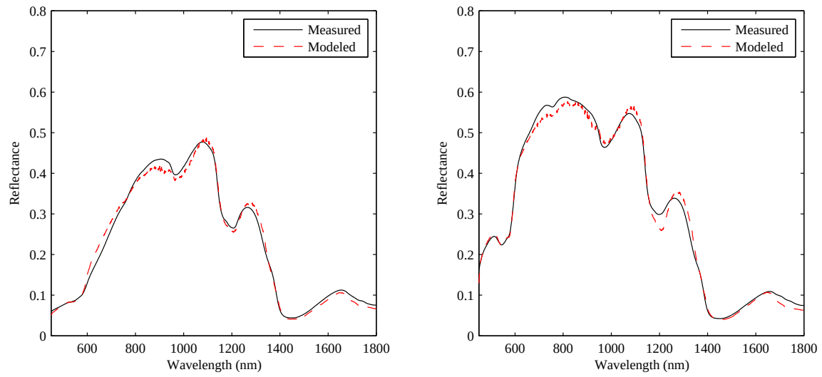
Figure 96: Comparison of model and measured living skin reflectance for sample 23 and 24.
