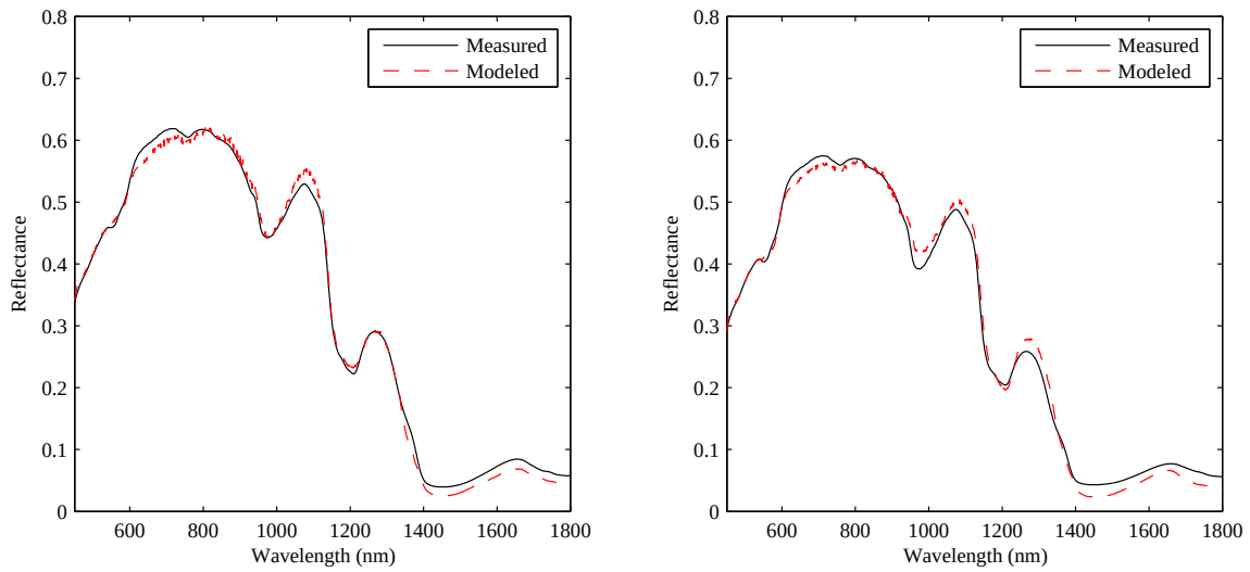
Figure 112: Comparison of model and measured cadaver skin reflectance for sample 55 and 56.
