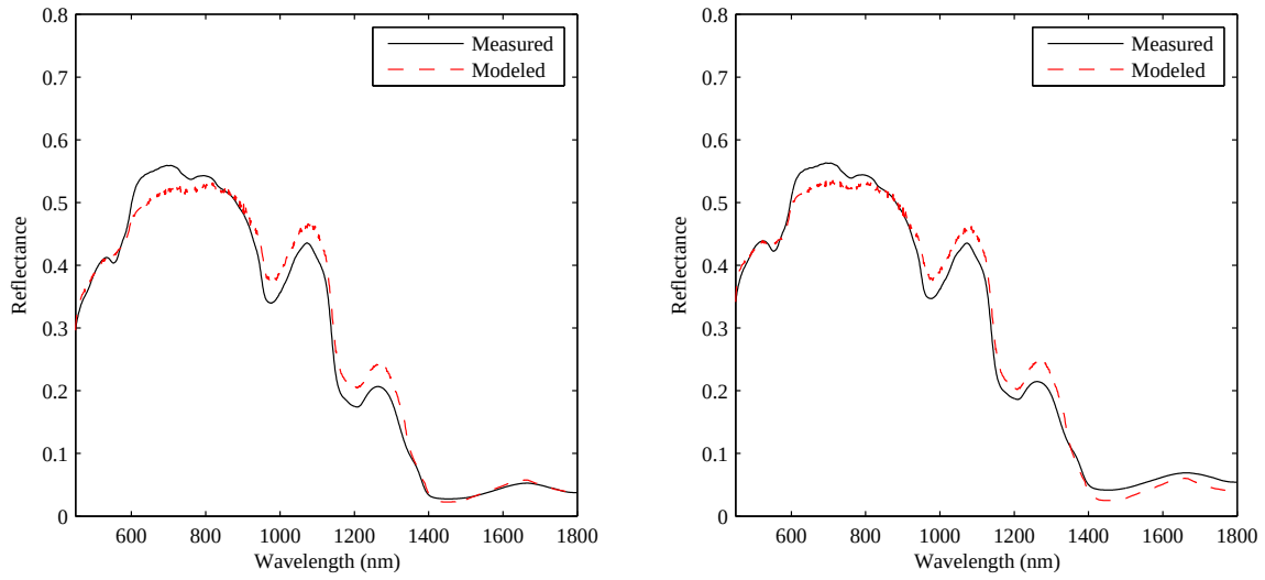
Figure 111: Comparison of model and measured cadaver skin reflectance for sample 53 and 54.
