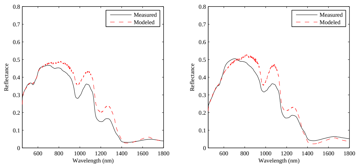
Figure 108: Comparison of model and measured cadaver skin reflectance for sample 47 and 48.
