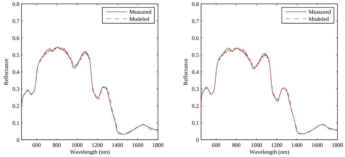
Figure 91: Comparison of model and measured living skin reflectance for sample 13 and 14.
