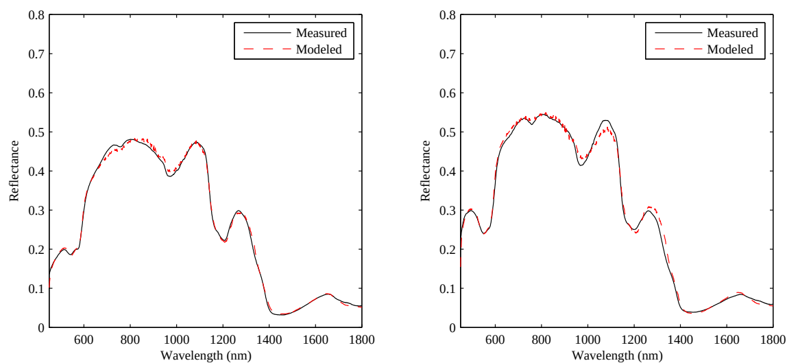
Figure 88: Comparison of model and measured living skin reflectance for sample 7 and 8.
