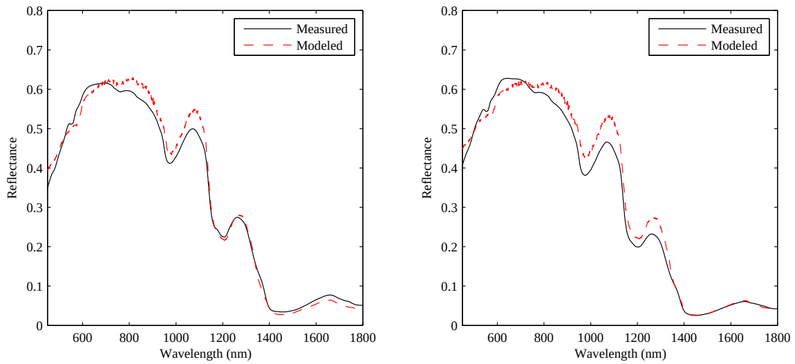
Figure 104: Comparison of model and measured cadaver skin reflectance for sample 39 and 40.
