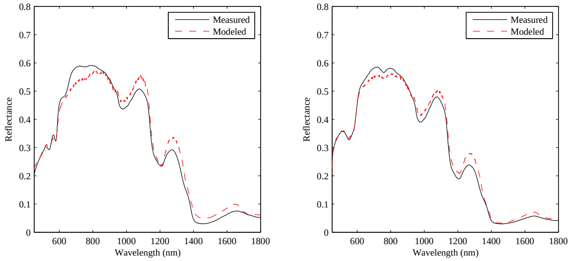
Figure 103: Comparison of model and measured cadaver skin reflectance for sample 37 and 38.
