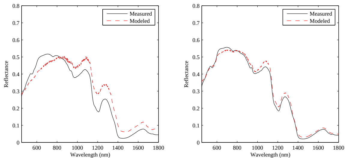
Figure 101: Comparison of model and measured cadaver skin reflectance for sample 33 and 34.
