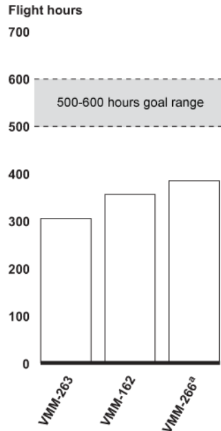
Figure 6: Iraq-Deployed MV-22 Squadrons' Average Engine Time on Wing
