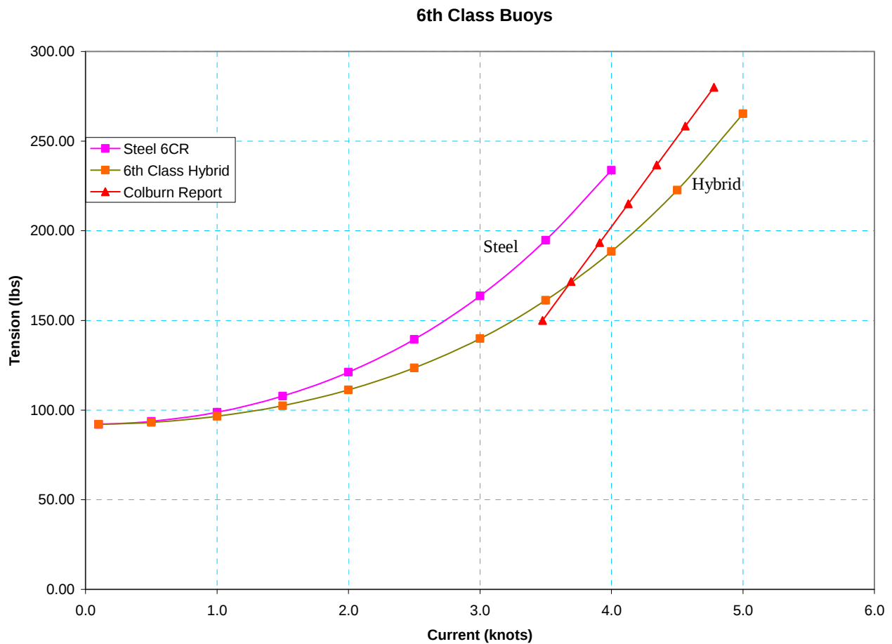
Figure 14. 6 th Class buoy comparison: current vs. mooring tension.
