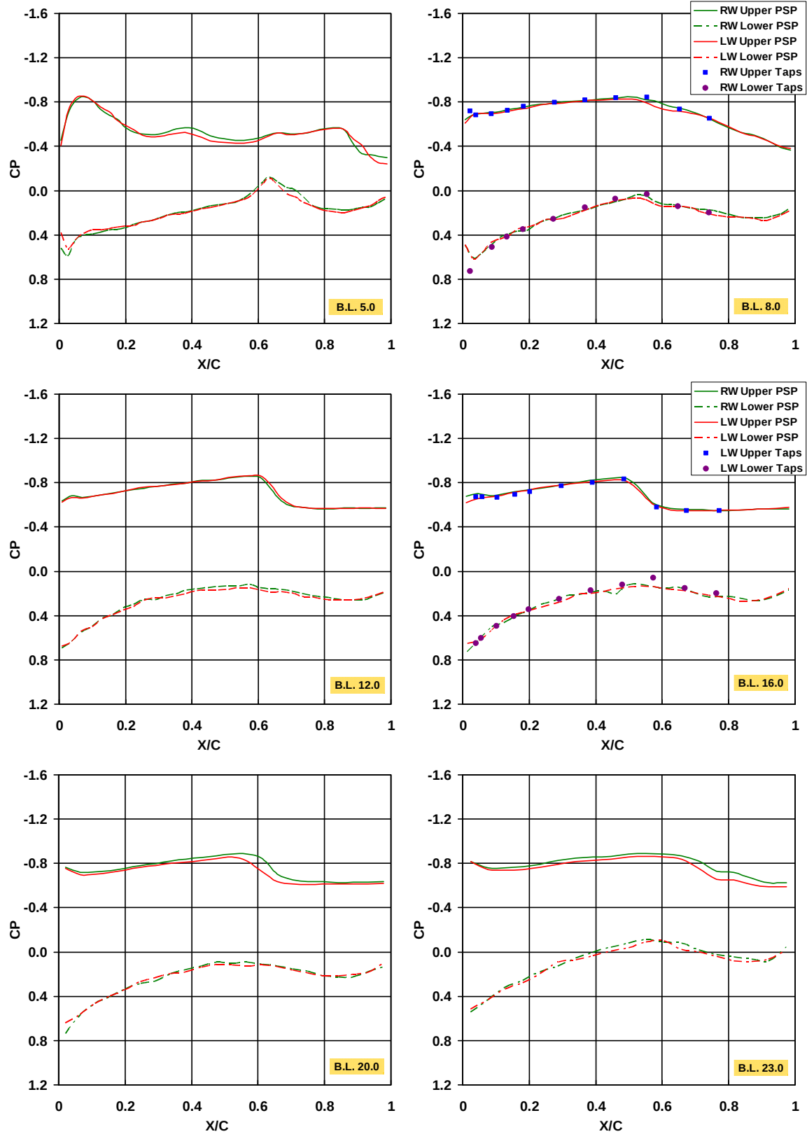
d. Alpha 10 deg. Figure 11. Continued.
