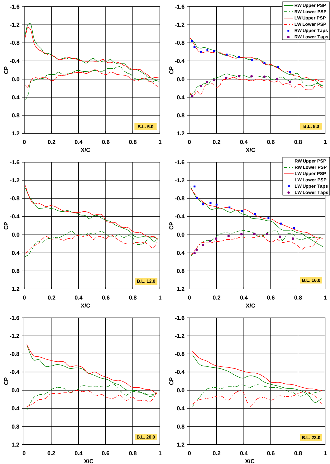
b. Alpha 4 deg. Figure 8. Continued.
