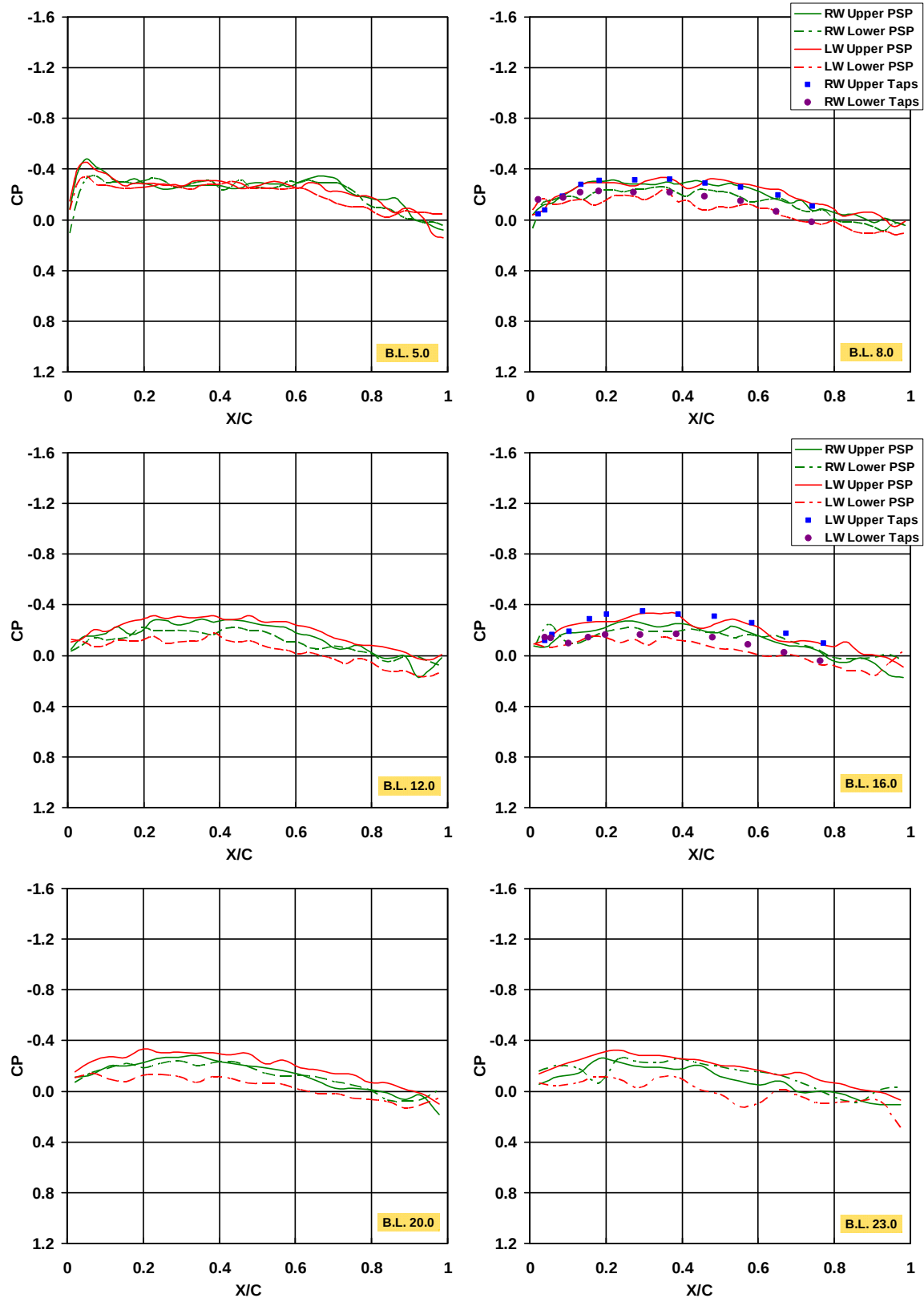
Figure 8. Mach Number 0.4 Wing Pressure Coefficient Comparison.
