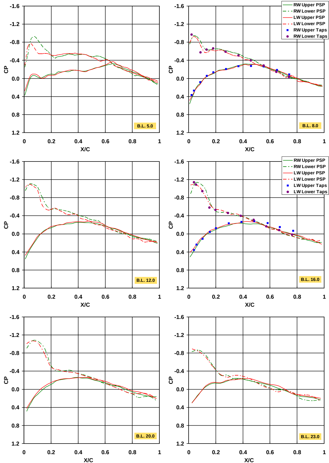
Figure 9. Mach Number 0.8 Wing Pressure Coefficient Comparison.
