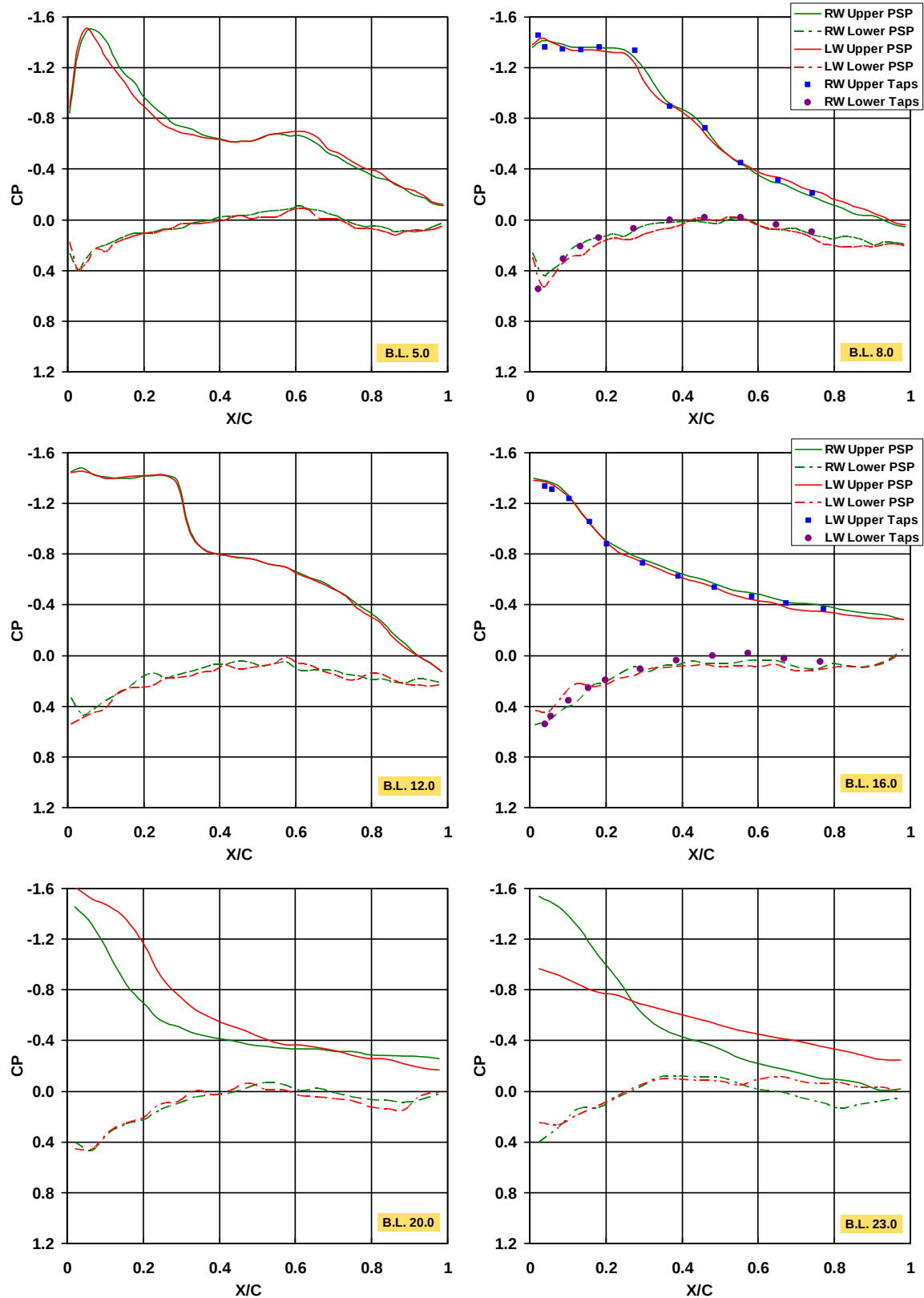
d. Alpha 7 deg. Figure 9. Continued.
