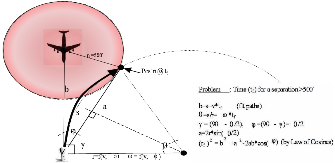
Figure 21. Avoidance Maneuver, General Solution.
