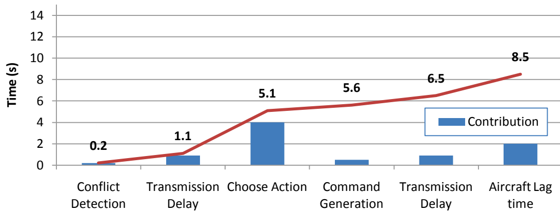
Figure 24. Time to React to a Collision Threat, Automated Detection
