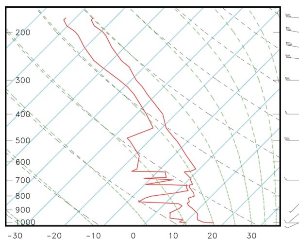
FIG. 5. SkewT/log-P thermodynamic sounding for Vandenberg, CA, for 0000 UTC 29 October 2000. The horizontal wind speed ( \text{m s}^{-1} ) and direction are shown to the right. One full wind barb corresponds to 5 \text{ m s}^{-1} and a flag denotes 25 \text{ m s}^{-1} .
