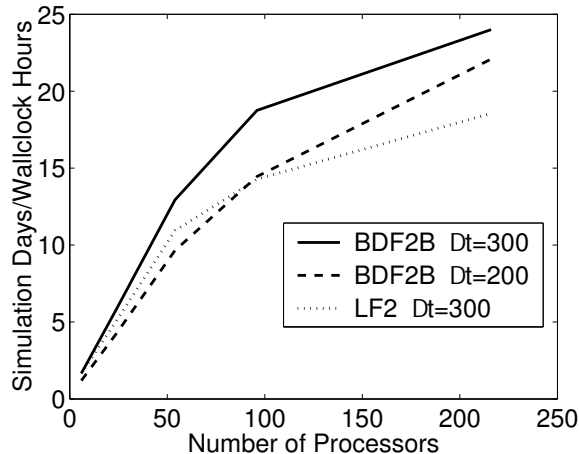
Figure 5. Efficiency of BDF2 and LF2 semi-implicit methods for NSEAM T249 N6 L30 on an IBM SP4 (P690 with 1.3 GHz clockspeed).
