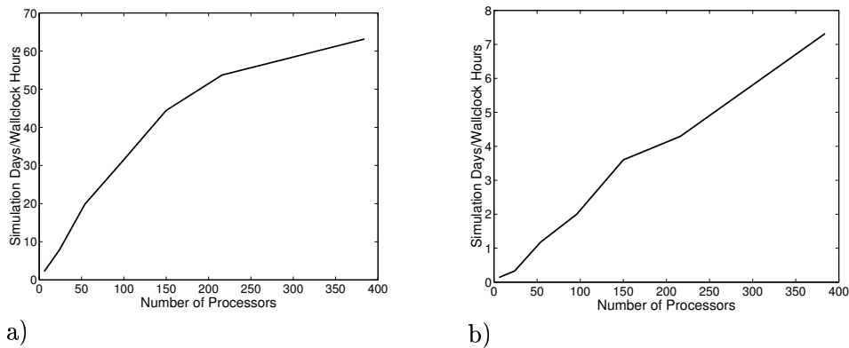
Figure 7. Simulation days per wallclock hours for the dynamical core of NSEAM (using BDF2B) on an IBM SP4 (P655 with 1.7 GHz clockspeed) using a) T249 N6 L30 with \Delta t = 300 seconds and b) T498 N6 L60 with \Delta t = 150 seconds.
