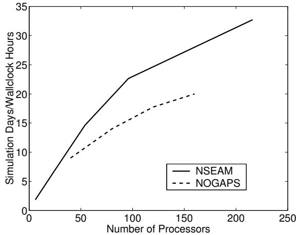
Figure 6. Simulation days per wallclock hours for the dynamical cores of NSEAM (T249 N6 L30 using BDF2B) and NOGAPS (T239 L30) on an IBM SP4 (P690 with 1.3 GHz clockspeed) using \Delta t = 300 seconds. (The performance data for NOGAPS is courtesy of Tim Hogan.)
