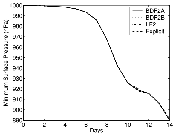
Figure 12. Jablonowski-Williamson Baroclinic Instability: The minimum surface pressure (hPa) as a function of days for NSEAM T185 N8 L26 using the semi-implicit BDF2A with \Delta t = 135 seconds (solid line), semi-implicit BDF2B method with \Delta t = 180 seconds (dotted line), semi-implicit LF2 method with \Delta t = 270 seconds (dashed-dotted line), and the explicit LF2 method with \Delta t = 42 seconds (dashed line).
