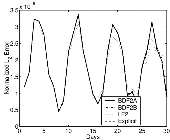
Figure 10. Jablonowski-Williamson Balanced Initial State: The normalized \pi L_2 error as a function of days for NSEAM T185 N8 L26 using the semi-implicit BDF2A method with \Delta t = 135 seconds (solid line), semi-implicit BDF2B method with \Delta t = 180 seconds (dashed-dotted line), semi-implicit LF2 method with \Delta t = 270 seconds (dotted line), and the explicit LF2 method with \Delta t = 42 seconds (dashed line).
