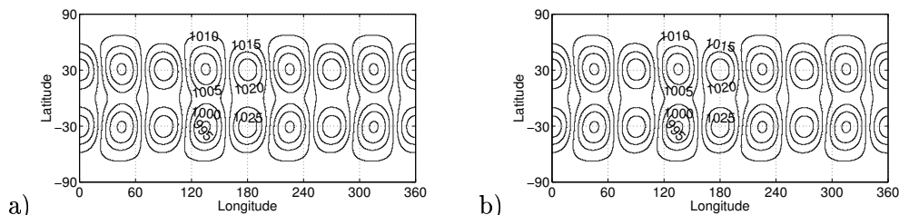
Figure 8. Rossby-Haurwitz Wave Number 4: The surface pressure contours in hPa for NSEAM T185 N8 L24 using the a) BDF2B and b) LF2 semi-implicit time-integrators.
