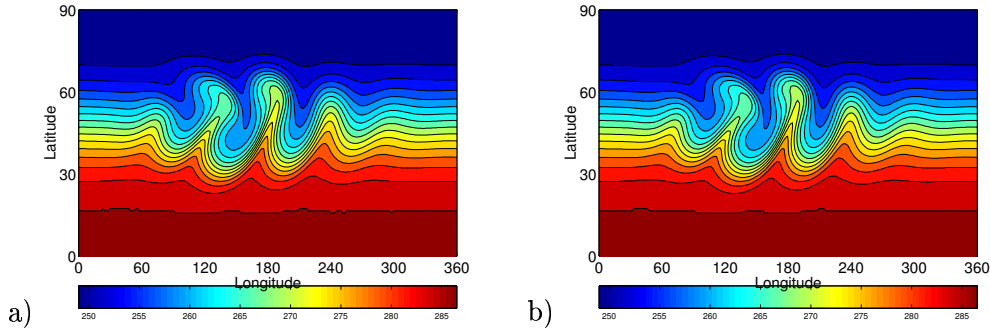
Figure 9. Polvani et al. Test Case: The surface temperature of NSEAM T74 N8 L20 after 12 days using the a) BDF2B and b) LF2 semi-implicit time-integrators.
