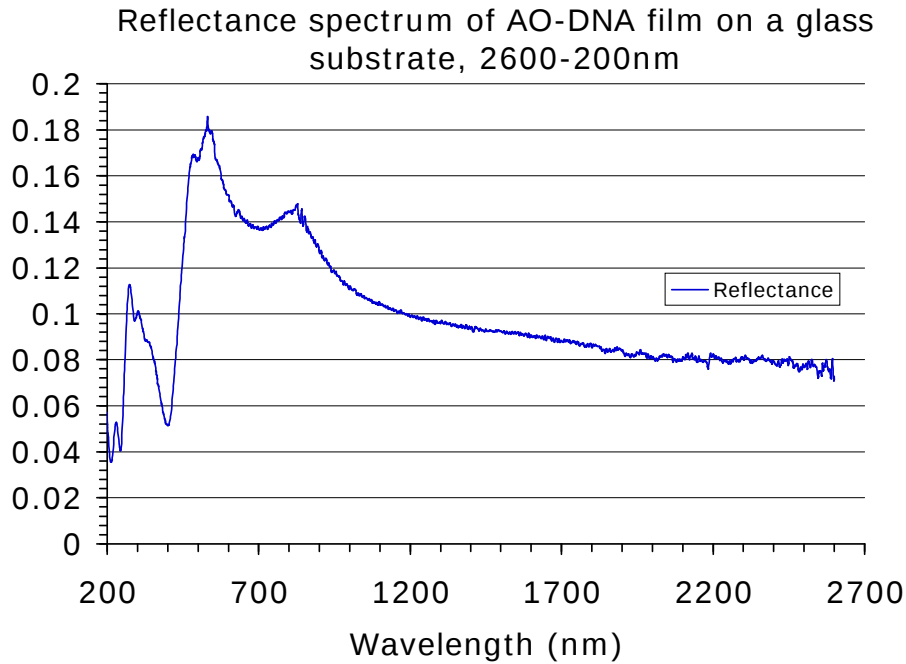
Fig. 3 shows reflectance spectrum in the film of DNA doped with Acridine Orange. R_{\max} is at 530nm, R_{\min} at 400nm. The additional reflectance maximum at about 850 is an artifact.
