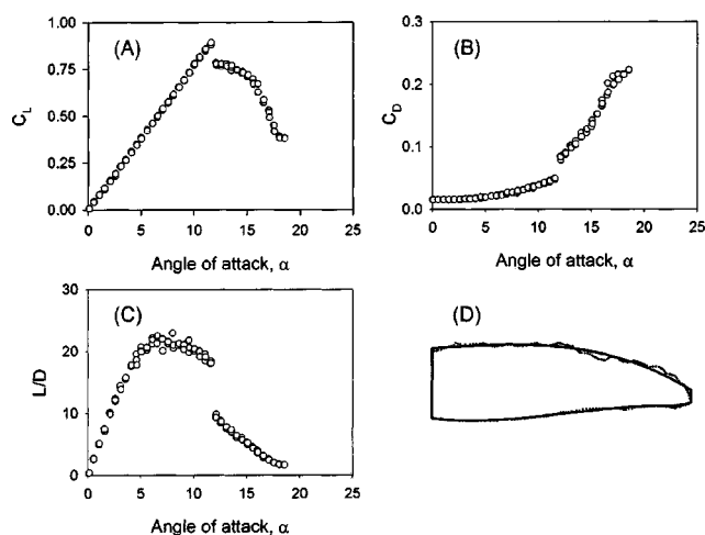
FIG. 3. Lift and drag data for the smooth whale flipper model. (a) Wind tunnel measurement of the lift coefficient, C_L , shown as a function of the angle of attack, \alpha . (b) Drag coefficient, C_D , shown as a function of the angle of attack. (c) Aerodynamic efficiency, L/D , which quantifies the drag cost of producing lift, shown as a function of the angle of attack. (d) Planform profile of the smooth flipper model (solid line) superimposed on the actual flipper profile (dotted line). In this orientation, flow would progress from top to bottom. (a) and (b) show that stall occurs near \alpha \approx \pm 12^\circ .
