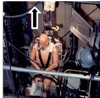
+Z: Runs were completed on both the horizontal accelerator (left) and vertical accelerator (right). +Z axial accelerations simulate aircraft ejection and ship shock.
