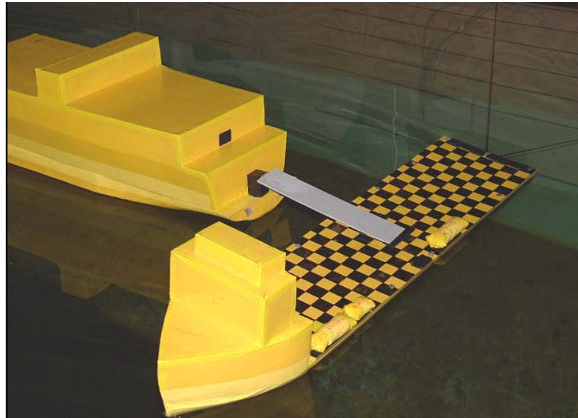
Figure 9 - Ramp Torsion
