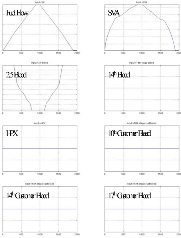
Figure 4 Training inputs
