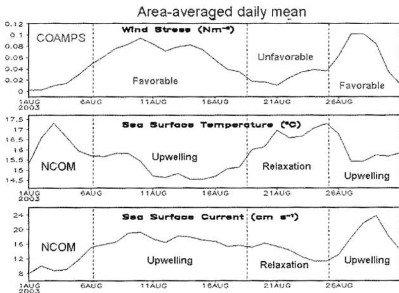
Fig. 4 Area-averaged daily mean for surface (a) wind stress, (b) temperature, and (c) current. The area is within 36.2\text{--}37.2^{\circ}\text{N} and 123\text{--}121.6^{\circ}\text{W}
