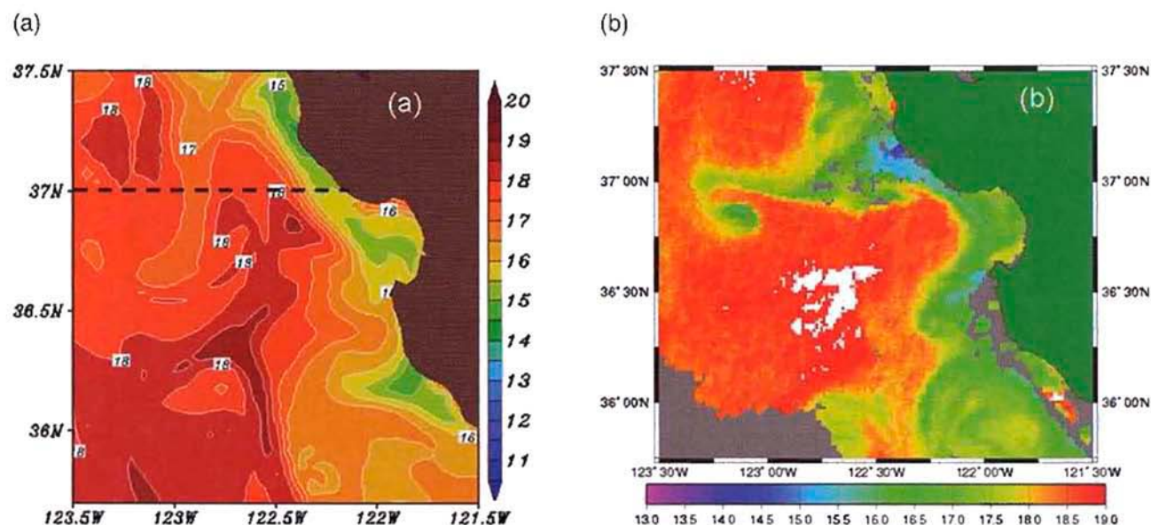
Fig. 9 (a) NCOM SST from 18 h forecast valid at 18Z August 24, 2003. (b) NOAA POES AVHRR HRPT SST at 1856Z August 24, 2003 (NOAA POES AVHRR, Courtesy NWS and NOAA Coastwatch)
