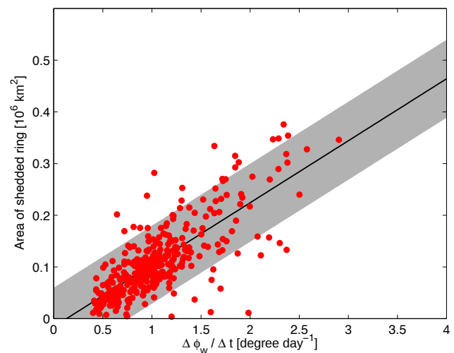
Fig. 4. The change in front location for loop occlusion events for the AG01 model (when \Delta\phi_w/\Delta t > 0.4 degree day ^{-1} ) versus the area of the associated ring being shed. The black line is the best linear fit, with the gray area denoting the 90% confidence band. The correlation coefficient of the data set is 0.77.
