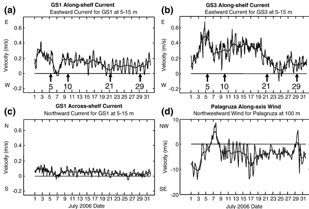
Fig. 5. Currents and winds for July (spanning MODIS images in Fig. 6). Eastward (along-shelf) current at (a) GS1 and (b) GS3, (c) northward current (across-shelf) at GS1 and (d) corresponding northwestward wind velocity component at Palagruza Island. Instantaneous sample values are plotted with 25-h cutoff period low-pass values (smooth solid line) superimposed.
