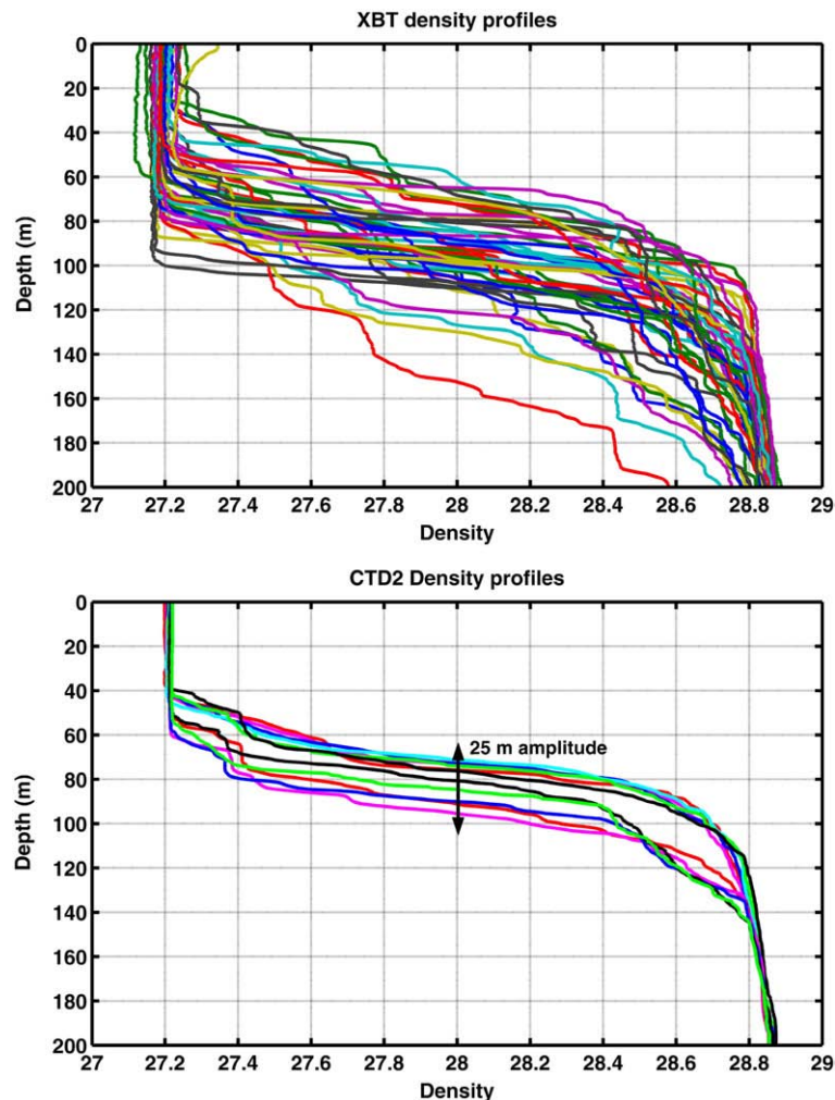
Fig. 4. Top, density profiles from all XBT probes (see Fig. 1 for locations) in the south of the strait (Ionian Sea) illustrating the variability in the water column due to the impact of internal waves. Bottom, density profiles measured by the lowered CTD probe at location ( 15^{\circ}34'04'' \text{ E} , 38^{\circ}03'04'' \text{ N} ). The pycnocline depth has a 25 m amplitude variability illustrating the occurrence of an internal wave event. Density units are “sigma-t”.
