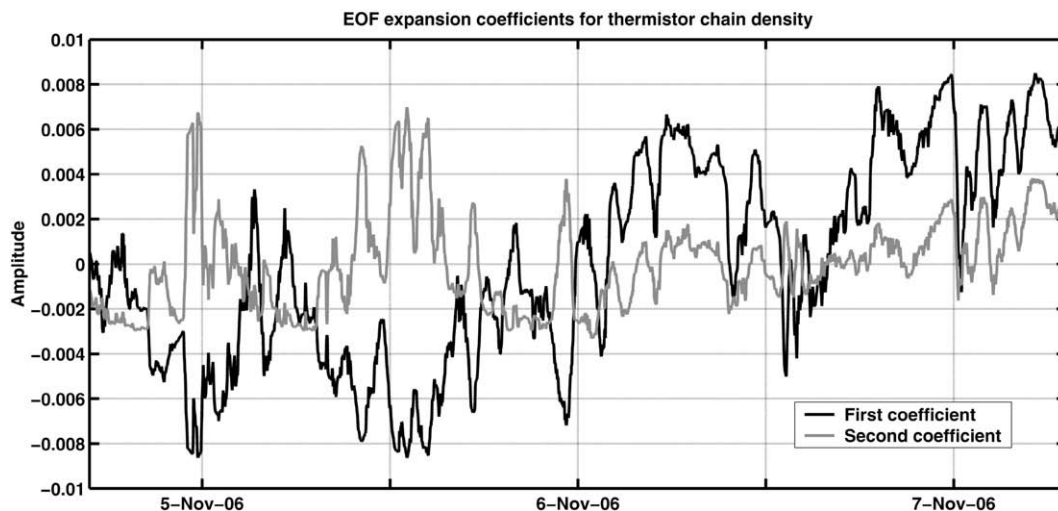
Fig. 8. Expansion coefficients for the first two EOF modes. The first expansion coefficient clearly represents the vertical oscillation of the pycnocline in time (compared with density contour 28.5 on Fig. 5). Both coefficients have stronger (absolute) values during internal wave events.
