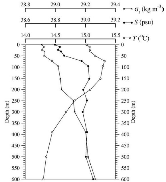
Fig. 9. Vertical profiles of T , S and density at 37.2°N, 23.7°E on 4 January 1990. The T and S profiles are from the WOD05 data set, and density was computed with UNESCO equation of state with no pressure dependence, as explained in the text. Profiles were taken at the local time of 15 GMT.
