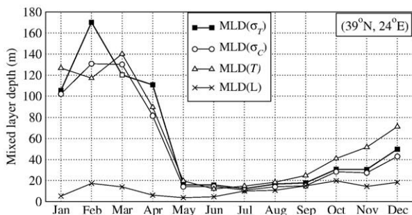
Fig. 8. The same as Fig. 7 but at 39°N, 24°E.
