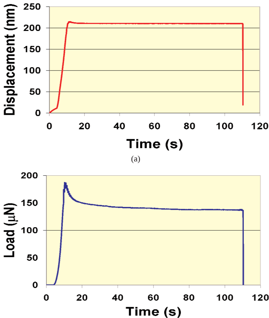
Fig. 4. Displacement-time (a) and corresponding force-time (b) for an indentation stress-relaxation test using a force-controlled system and feedback to control displacement.
