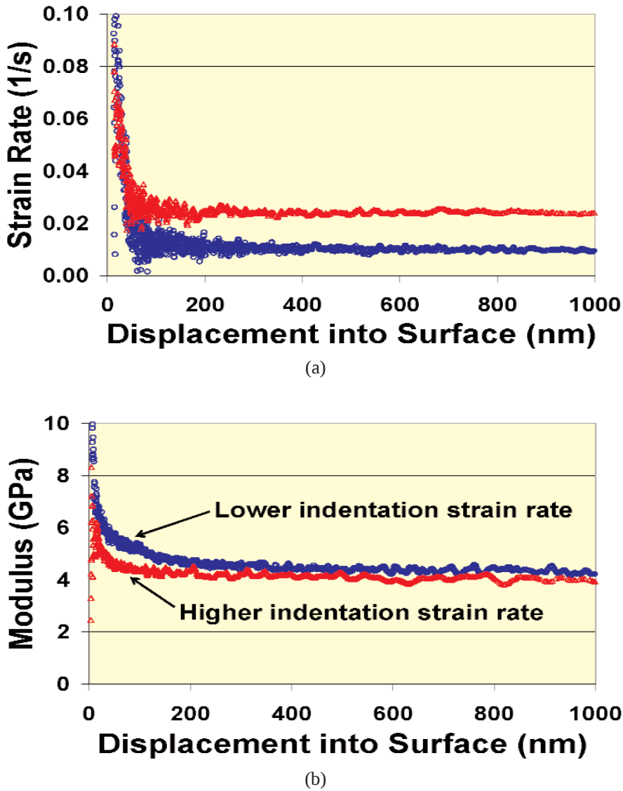
Fig. 10. Plots of indentation strain rate, \dot{\epsilon}_i , estimated by the ratio \dot{P}/P (a) and indentation modulus (b) as a function of depth, h , for a constant \dot{P}/P test using a Berkovich indentation tip to penetrate a polystyrene sample. Data for one test each at two different rates are shown. Differences in the modulus data are estimated to be within the measurement uncertainty.
