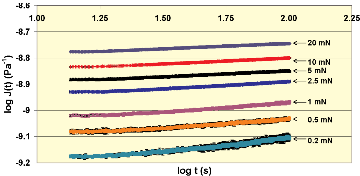
Fig. 11. Log-log plot of creep compliance, J(t) , as a function of time, t , for an indentation creep experiment on epoxy using a rounded conical tip (manufacturer-determined tip radius of 10 \mu\text{m} ). Error bars shown represent an estimated standard deviation ( k = 1 ).
