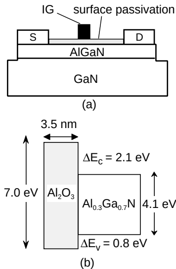
Fig.5: \text{Al}_2\text{O}_3 IG-HFET.
