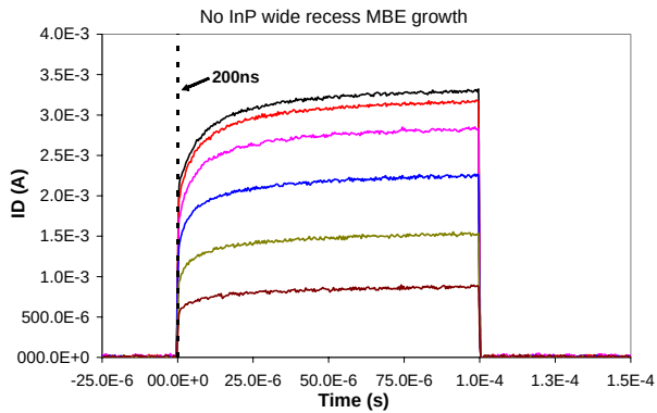
Fig 5: Gate lag turn on current pulses (100μs wide) for (A) (on the left) and (C) (on the right) devices at different bias conditions
