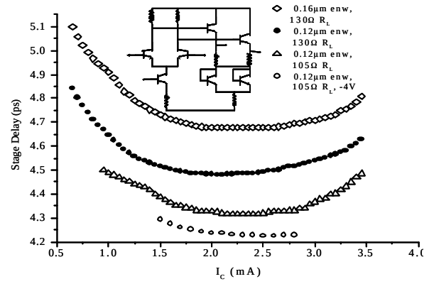
Figure 1. Stage delay vs. collector current (tail current) for ring oscillators fabricated with 0.12 and 0.16 \mu\text{m} emitter width NPN and different load resistors ( R_L ).
