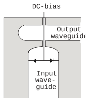
Fig. 2 THz multiplier topology [8]. The electric field is in the plane of the figure
