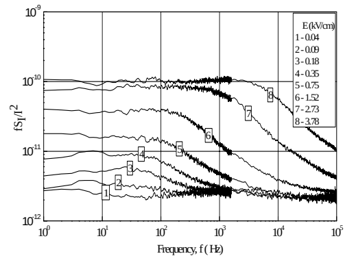
Fig. 2. Spectra of the normalized current noise for different values of the electric field E measured at T=300 K for the device with the channel length of 25 μm and the width of 100 μm.
