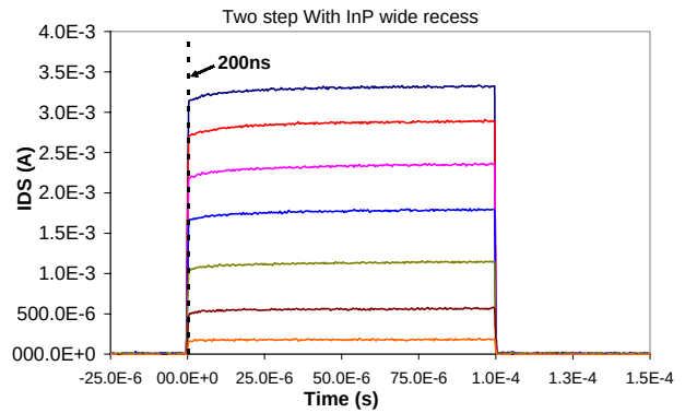
Fig 5: Gate lag turn on current pulses (100μs wide) for (A) (on the left) and (C) (on the right) devices at different bias conditions
