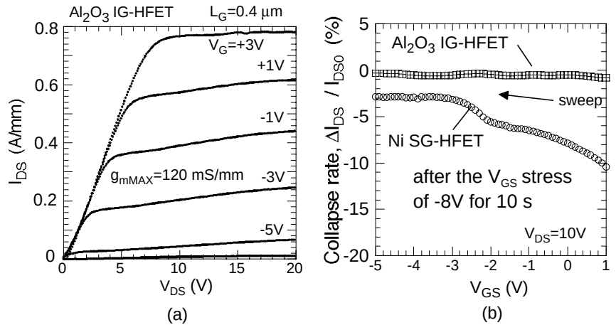
Fig.6: (a) Drain I-V characteristics and (b) percentage collapse values.
