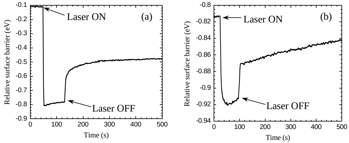
Fig. 1 Surface barrier transients caused by switching an UV laser ON and OFF for an (a) unpassivated and (b) \text{SiN}_x passivated AlGaIn/GaN heterostructure (35% Al, 250 \text{\AA} barrier thickness) grown on Sapphire.
