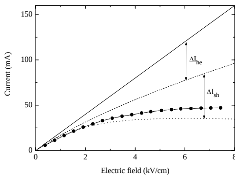
Fig. 1. The result of calculation I vs E for the device with channel length of 25 μm and width of 100 μm. Solid line is ohmic I-E curve, arrows show current decrease due to hot-electron (ΔI he ) and self-heating (ΔI sh ). Circles are experimental data measured at 300 K.
