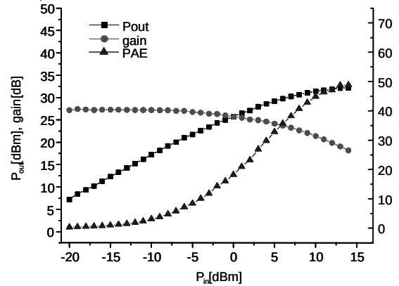
Fig. 9: Pa-PO9981 VSAT Ka-Band PA – PPH25 (2.47 mm 2 )
