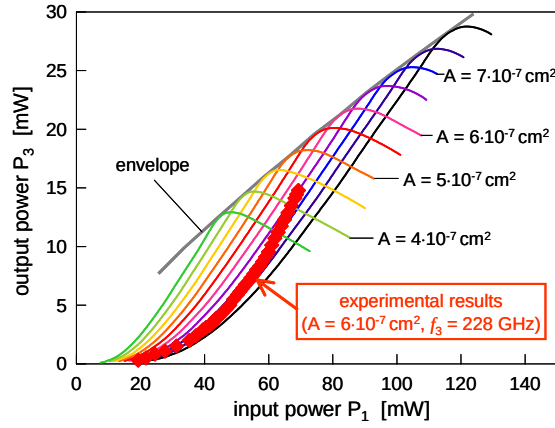
Fig. 2: Calculated output power P_3 versus input power P_1 of ASVs with different device areas ( f_1 = 76 GHz, f_3 = 228 GHz, R_{\text{CIRCUIT LOSS}} = 0.8 \Omega )
