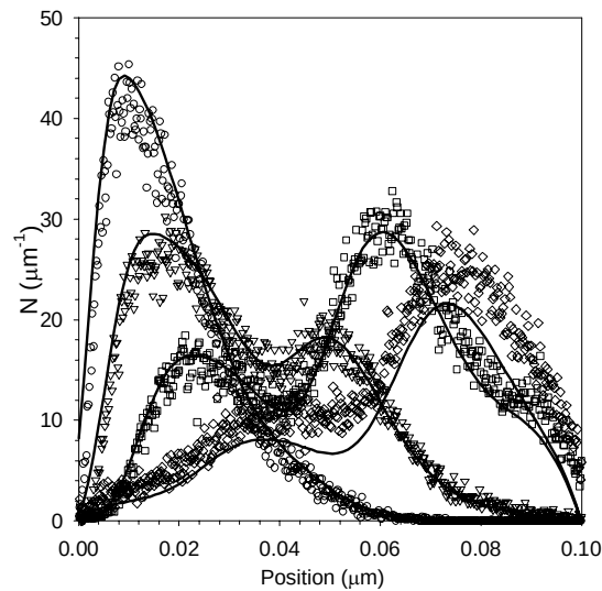
Figure 2: Electron concentrations (lines) for a 0.1 \mu\text{m} depletion region width thick p-i-n structure at F = 762 \text{ kV/cm} at four different times (0.1 ps (circles), 0.2 ps (triangles), 0.4 ps (squares) and 0.8 ps (diamonds)) computed using the bipolar FPE equation. The symbols represent the results from an equivalent bipolar MC simulation.
