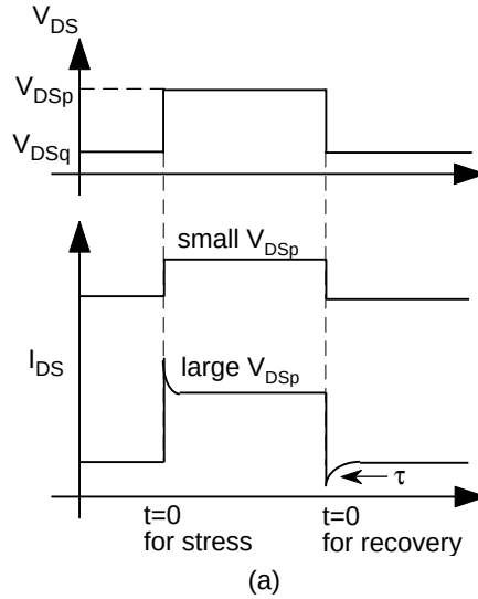
Fig.2: (a) Pulse waveforms of gateless HFET and (b) Arrhenius plots of \tau for emission.
