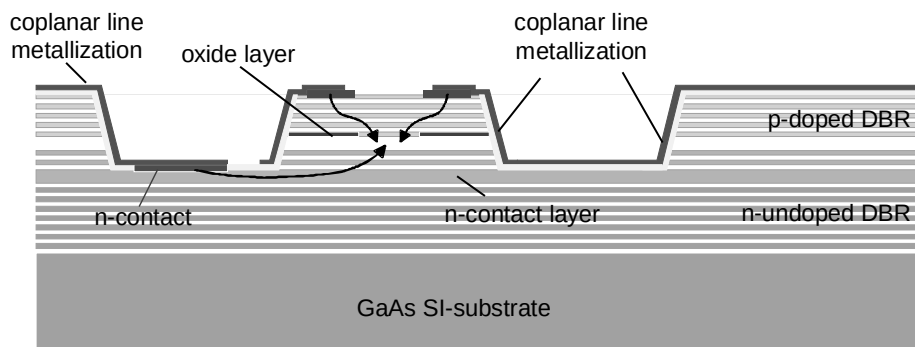
Figure 1: Cross-sectional schematic of a VCSEL structure designed for high speed operation.
