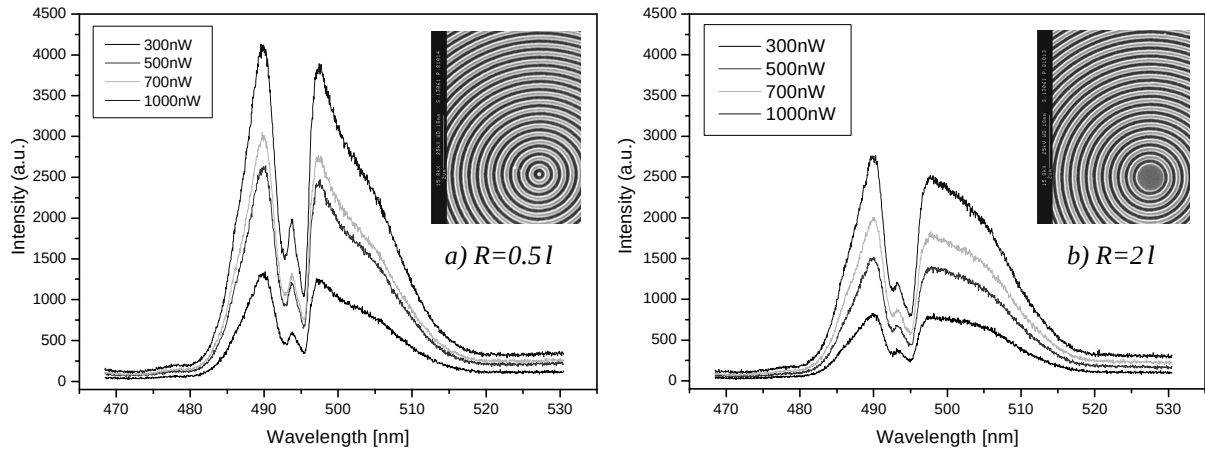
Fig. 3: SEM picture of a circular grating and its PL graph below lasing threshold. a) R = 0.5l and b) R = 2l .
