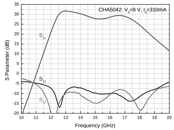
Fig. 7: 29-dBm Ka-band VSAT PA – PPH25x (1.9mm 2 - CHA5042) V ds = 8V / I ds = 310mA
