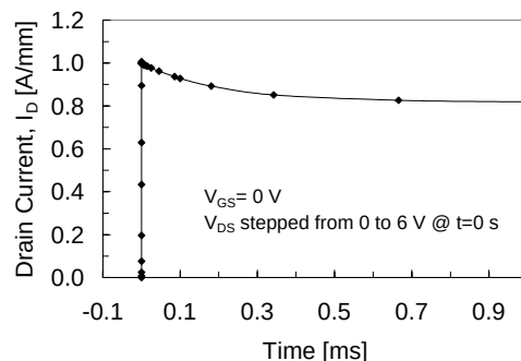
Fig. 8. Simulated I_D(t) transient following a V_{DS} turn-on step.
