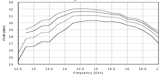
Fig. 8: 31-dBm Ku-band VSAT HPA – PPH25x ( 3.3mm 2 - CHA6042) (V ds = 6, 7, 8, and 9V respectively)
