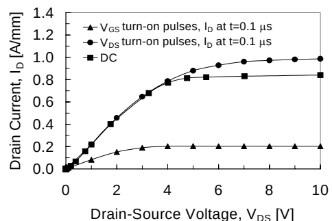
Fig. 6. Simulated I_D - V_{DS} characteristics obtained in DC and by pulsing either V_{GS} (from -5 V to the quoted V_{GS} ) or V_{DS} (from 0 to the x-axis value).
