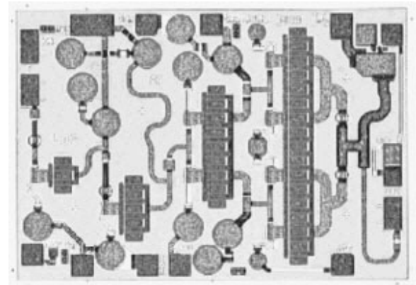
Fig. 9: Pa-PO9981 VSAT Ka-Band PA – PPH25 (2.47 mm 2 )
