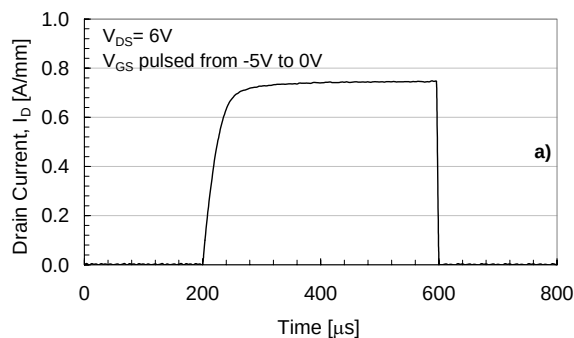
Fig. 3. a) Experimental I_D(t) transient in response of a V_{GS} turn-on pulse at V_{DS}=6 V.
