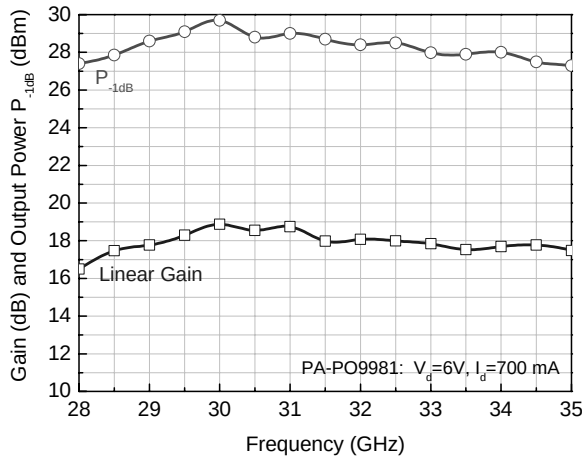
Fig. 10: VSAT Ka-Band PA – PPH25 (2.47 mm 2 ) V ds = 6V / I ds = 700mA
