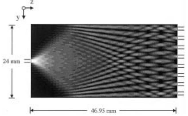
Fig. 2. Top view simulation of the electric field distribution of a 1 \times 8 power splitter.
