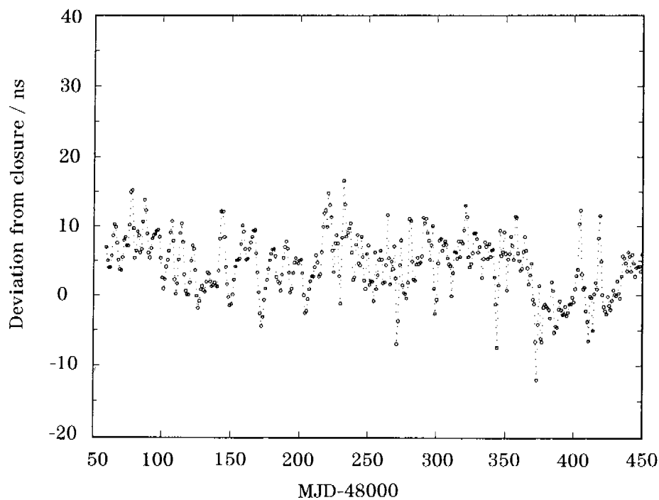
FIGURE 4: Deviation from closure around the world via OP, NIST and CRL with data corrected for precise ephemerides and measured ionospheric delay.
