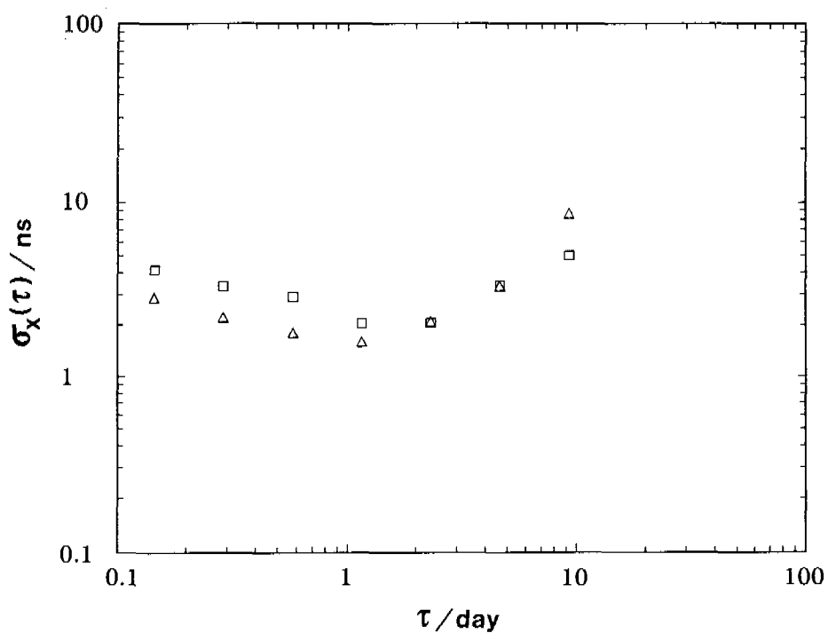
FIGURE 6: Square root of the time variance \sigma_x(\tau) of the link OP-NIST for data corrected using precise ephemerides and measured ionospheric delay over the periods MJD 48080 to 48160 (squares) and MJD 48375 to 48450 (triangles).
