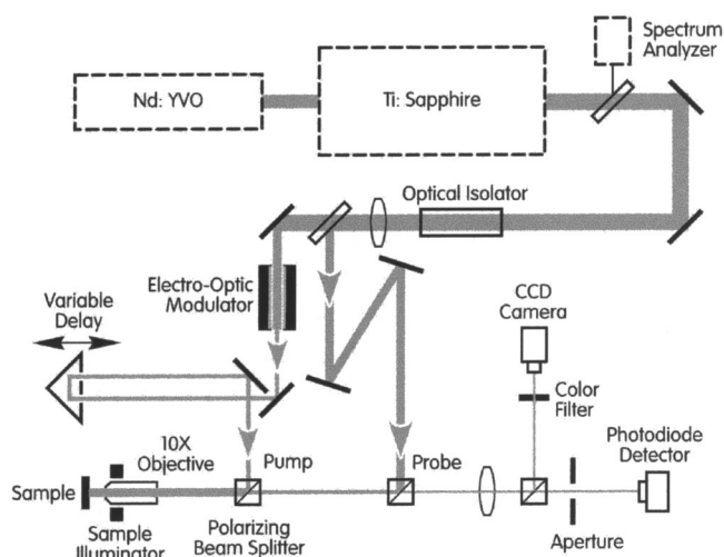
FIG. 16. Schematic of the TDTR and picosecond acoustics apparatus in use at the Laser Facility of the Frederick Seitz Materials Research Laboratory.
