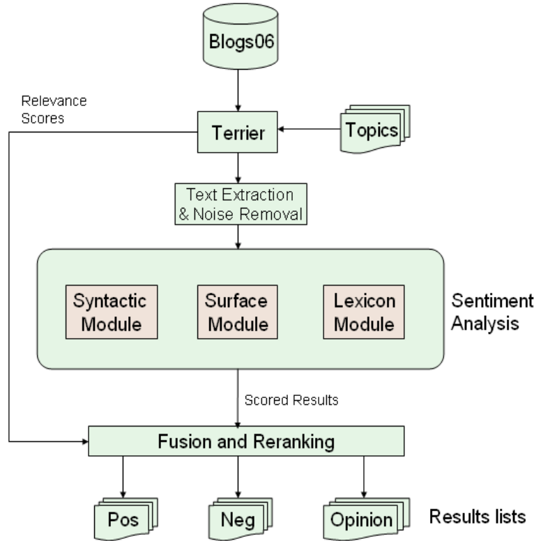
Figure 1: DCU's system architecture
