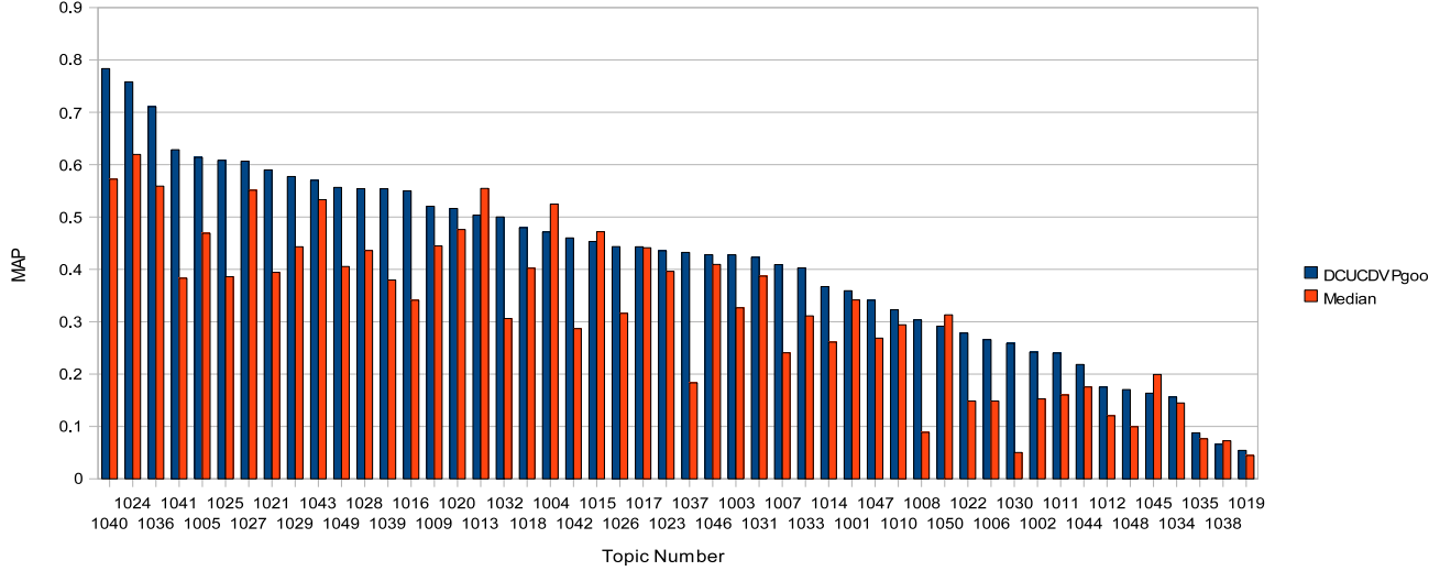
Figure 3: Per-topic MAP for DCU’s best-performing opinion run based on a distributed baseline, baseline4.
