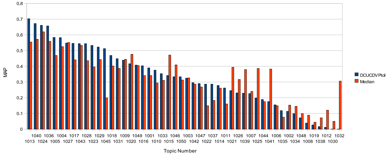
Figure 2: Per-topic MAP for the best-performing opinion run based on a non-distributed baseline, DCU's topic only baseline.
