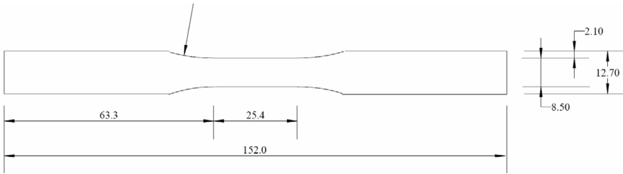
Figure 4: Specimen design
