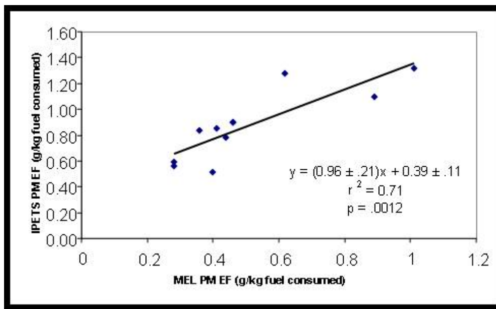
Figure 4-12. Comparison of ELPI PM with MEL PM emissions for the same engine exhaust.
