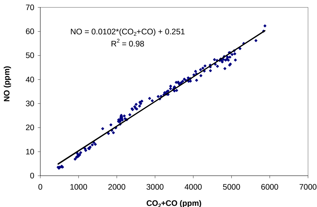
Figure 5-5. Correlation of FTIR NO with CO+CO 2 concentration over a sampling cycle
