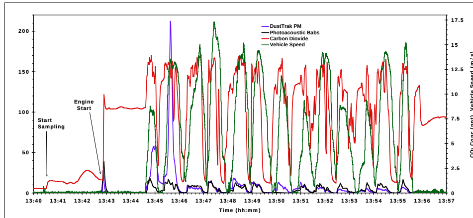
Figure 5-21. Raw on-board data for an MTVR driving five test loops (cycle #1).
