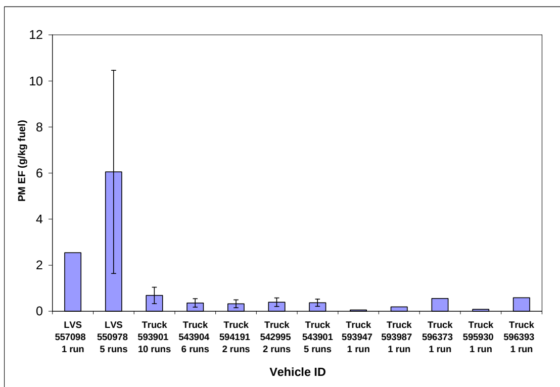
Figure 5-18. PM EF distribution for individual vehicles measured by IPETS. Error bars indicate the standard deviation of measurements of the same vehicle.
