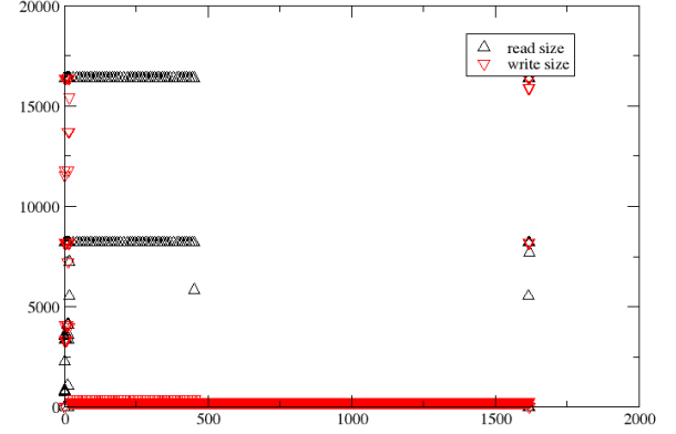
Fig. 7. Read/write I/O request sizes for pemodel as a function of time
