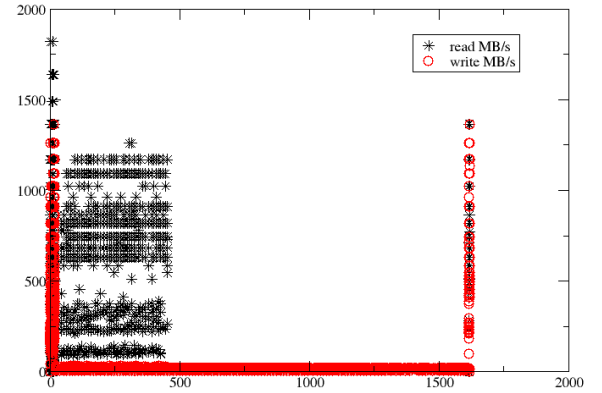
Fig. 8. Read/write throughput (in MB/s) for pemodel as a function of time - filesystem cache is enabled
