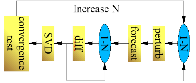
Fig. 3. The serial ESSE implementation
