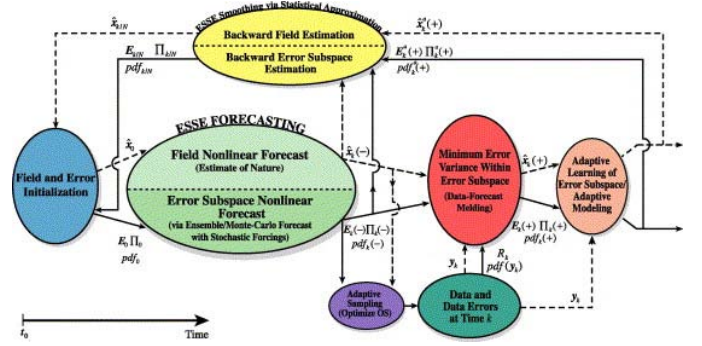
Fig. 2. The ESSE algorithm
