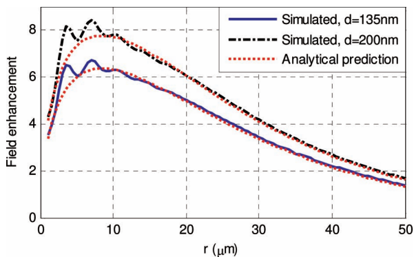
Figure 7. Numerically simulated field enhancement factor curves with respect to ring radius r for single ring plasmonic lens with different slit widths (135 and 200 nm, respectively) and their corresponding analytical predictions.
